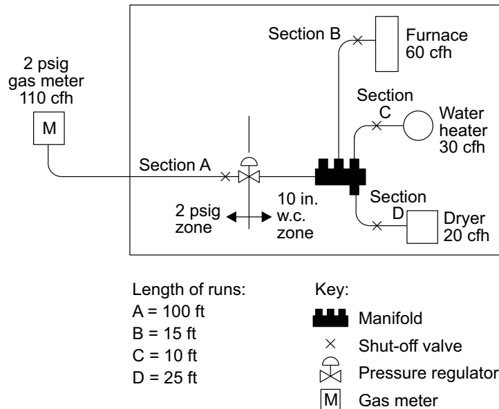
FIGURE CA106.2—PIPING PLAN SHOWING A CSST SYSTEM
