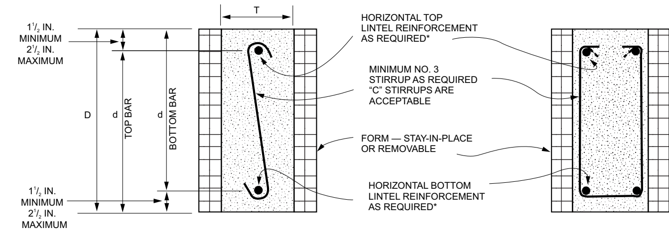
FIGURE R608.8(2)—LINTEL FOR FLAT WALLS
