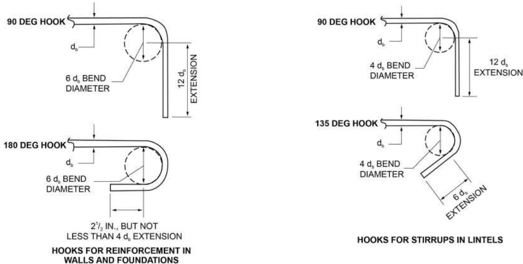
FIGURE R608.5.4(3)—STANDARD HOOKS
