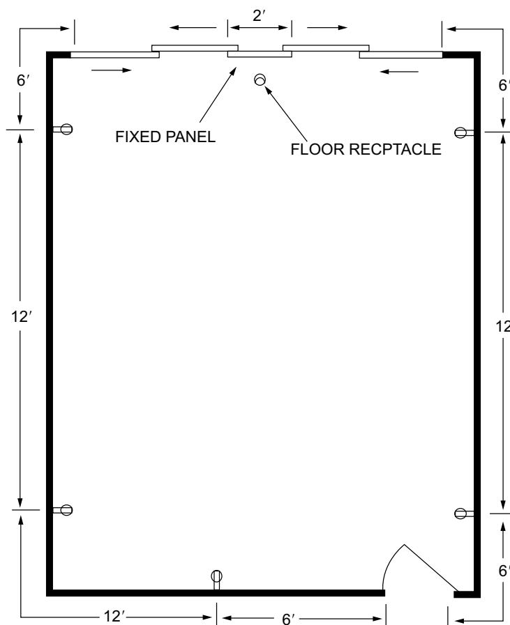
FIGURE E3901.2—GENERAL USE RECEPTACLE DISTRIBUTION
