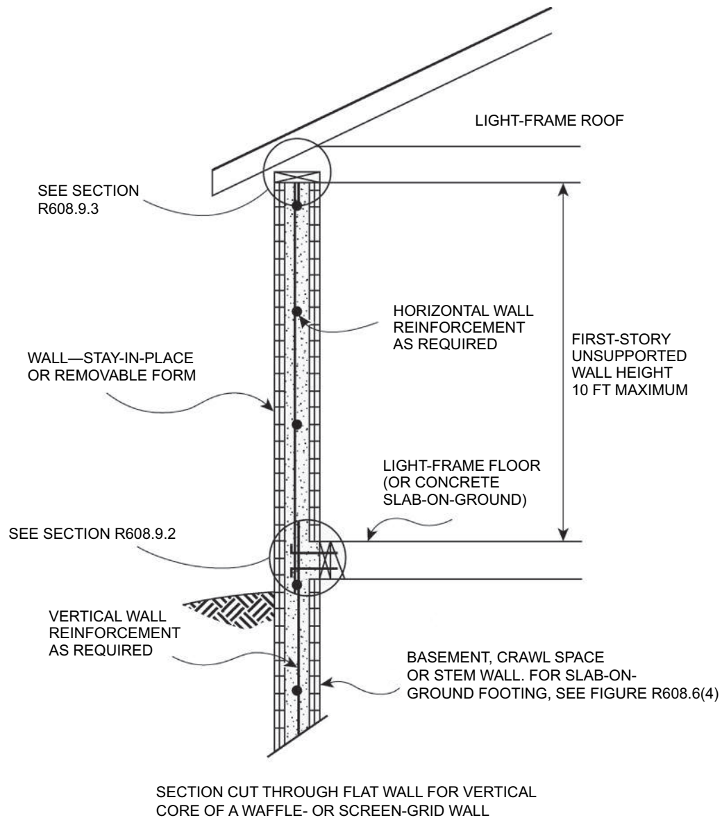
FIGURE R608.6(1)—ABOVE-GRADE CONCRETE WALL CONSTRUCTION ONE STORY
