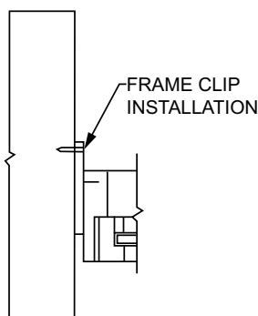
FIGURE R609.7.2(3)—THROUGH THE FRAME
