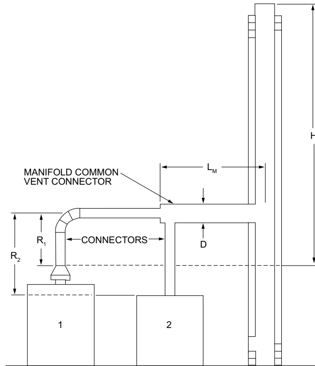
FIGURE CB102.5(6)—USE OF MANIFOLD COMMON VENT CONNECTOR
