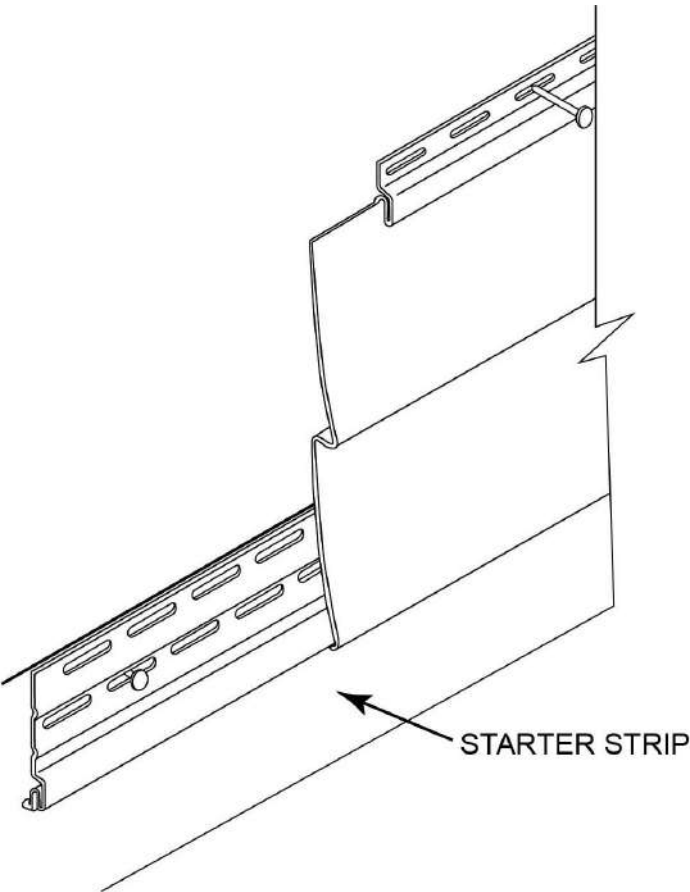
FIGURE R703.11.1.1(1)—TYPICAL STARTER STRIP a
