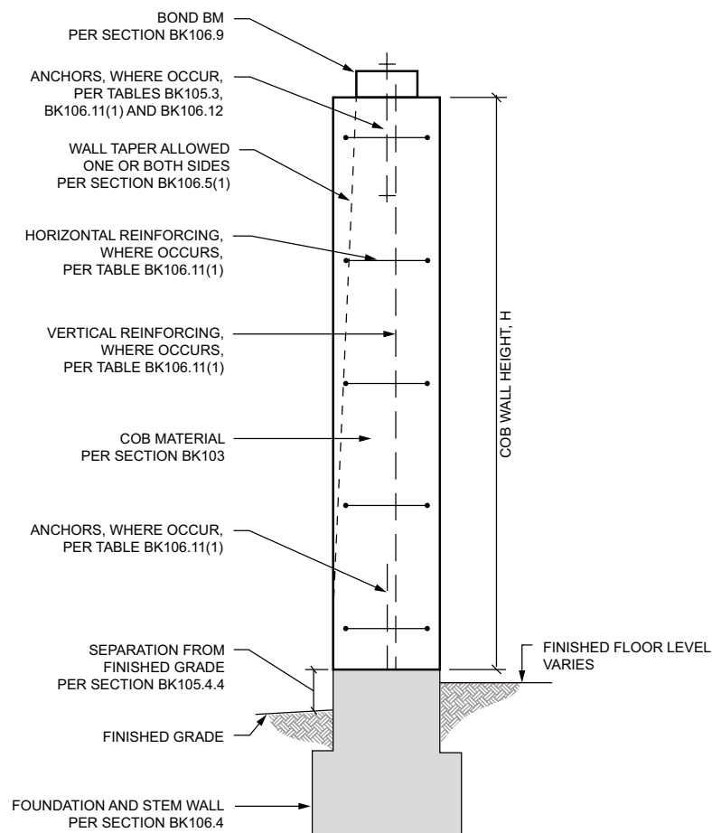
FIGURE BK101.4—TYPICAL COB WALL
