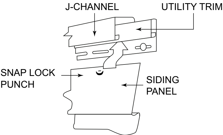
FIGURE R703.11.1.2 (1)—TYPICAL SNAP LOCK AND UTILITY TRIM a
