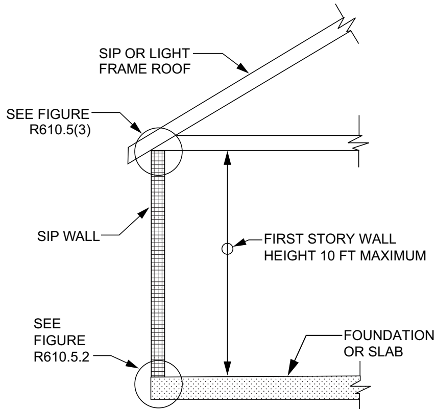
FIGURE R610.5(1)—MAXIMUM ALLOWABLE HEIGHT OF SIP WALLS
