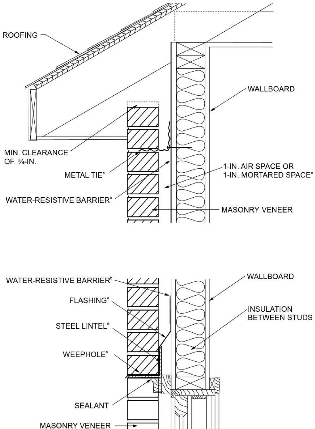
FIGURE R703.8(2)—TYPICAL MASONRY VENEER WALL DETAILS e
