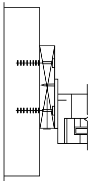
FIGURE R609.7.2(5)—THROUGH THE FLANGE
