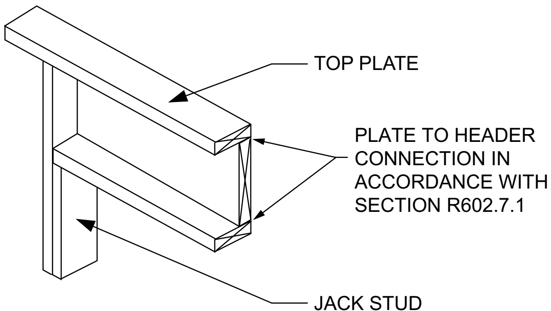
FIGURE R602.7.1(2)—ALTERNATIVE SINGLE-MEMBER HEADER WITHOUT CRIPPLE
