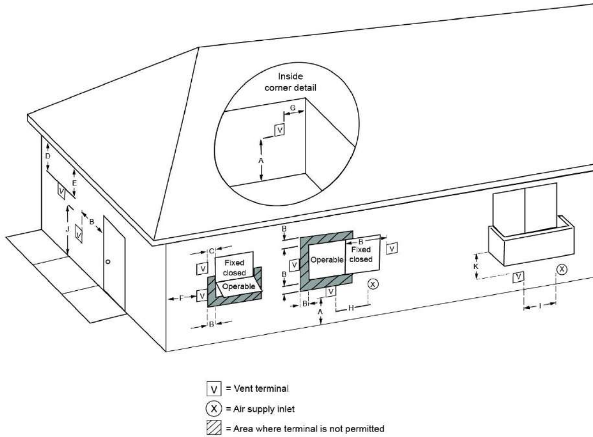
FIGURE G2427.8 (503.8)—THROUGH-THE-WALL VENT TERMINAL CLEARANCE
