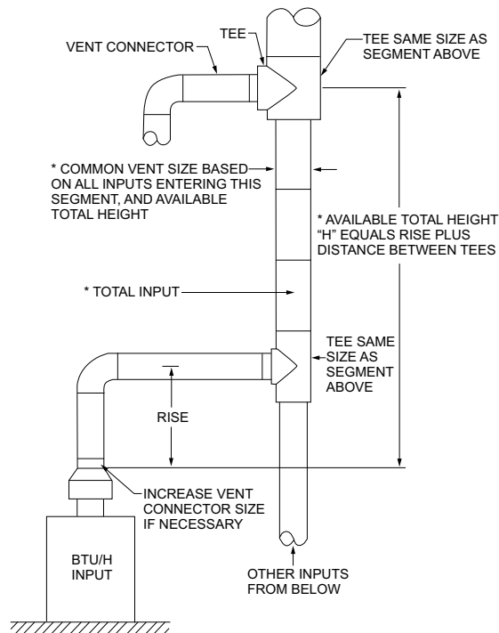
FIGURE CB102.5(8)—MULTISTORY GAS VENT DESIGN PROCEDURE FOR EACH SEGMENT OF SYSTEM
