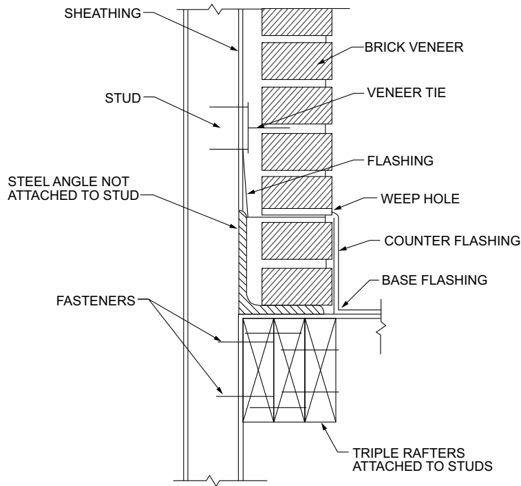
FIGURE R703.8.2.2(1)—EXTERIOR MASONRY VENEER SUPPORT BY ROOF MEMBERS
