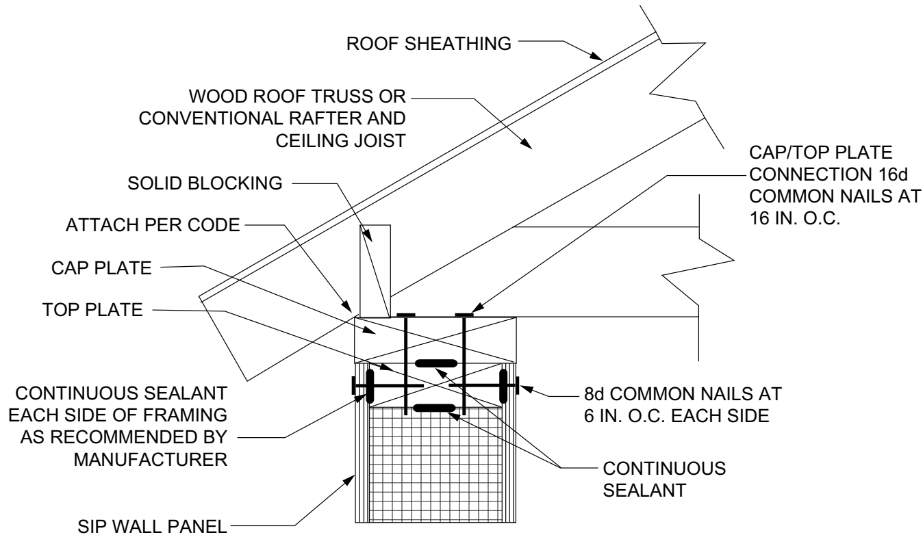
FIGURE R610.5(3)—TRUSSED ROOF TO TOP PLATE CONNECTION
