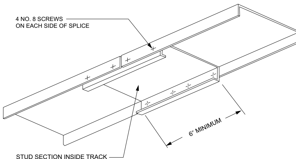
FIGURE R603.3.5—TRACK SPLICE
