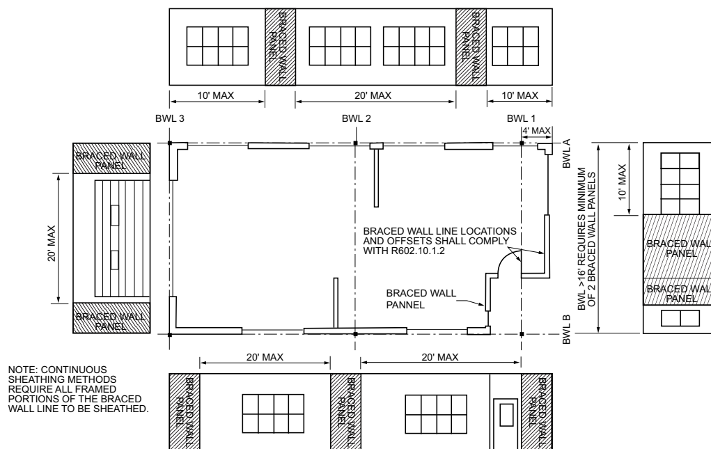
FIGURE R602.10.2.2—LOCATION OF BRACED WALL PANELS
