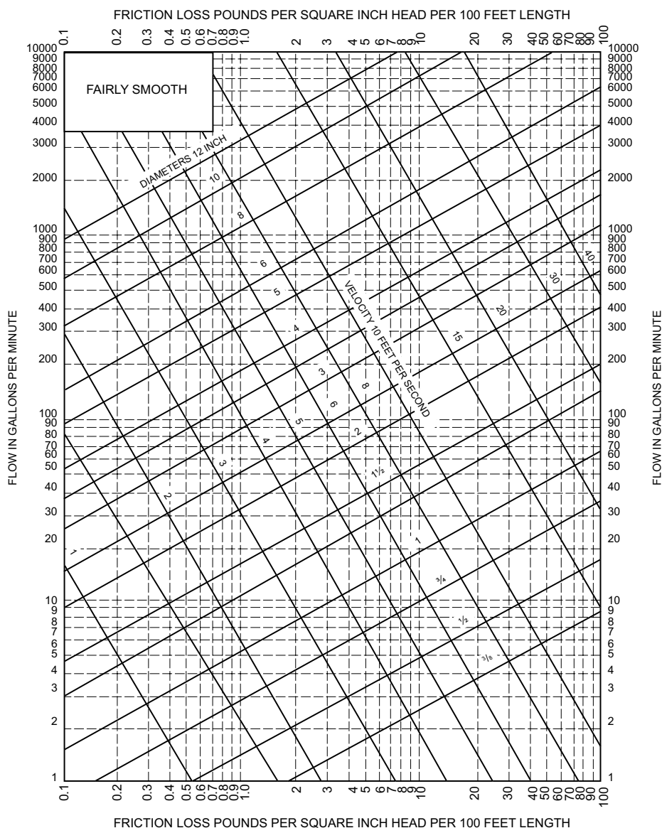
FIGURE CF103.3(5)—FRICTION LOSS IN FAIRLY SMOOTH PIPE a
