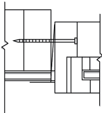
FIGURE R609.7.2(6)—THROUGH THE FLANGE
