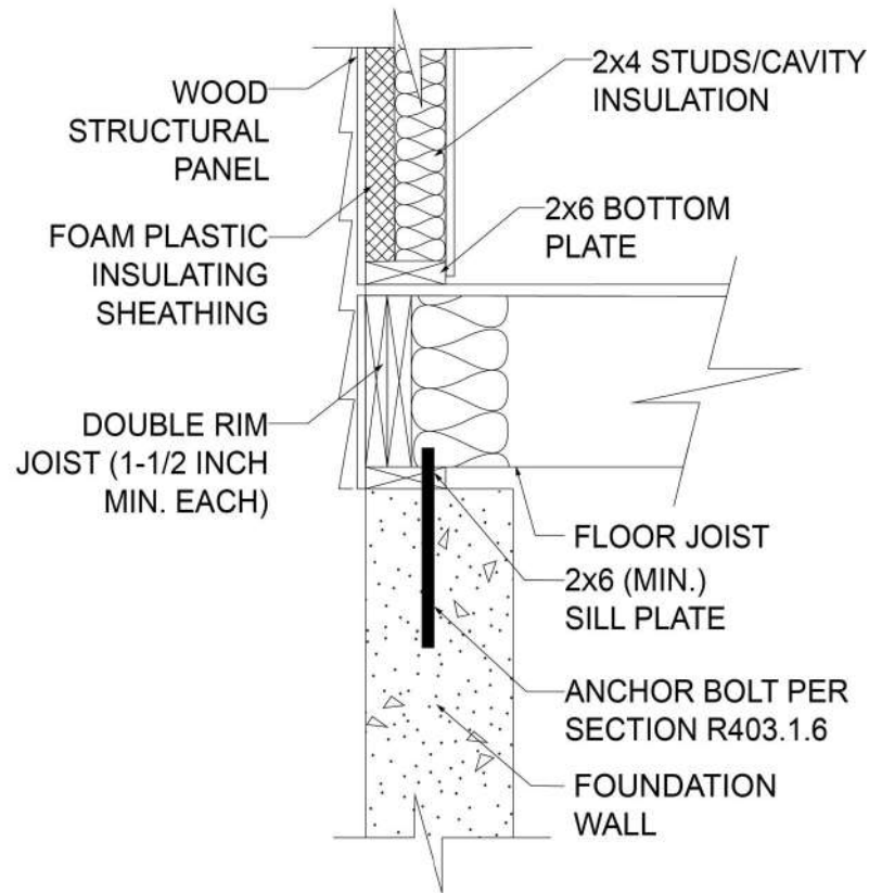
FIGURE BN102.4(1)—RIM JOIST CONSTRUCTION FOR EPW—DOUBLE MEMBER
