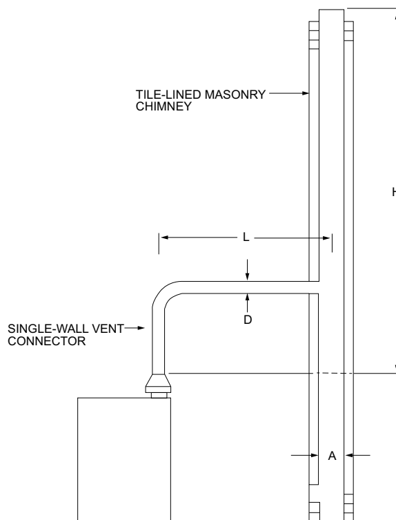
FIGURE CB101.4(4)—VENT SYSTEM SERVING A SINGLE APPLIANCE USING A MASONRY CHIMNEY AND A SINGLE-WALL METAL VENT CONNECTOR
