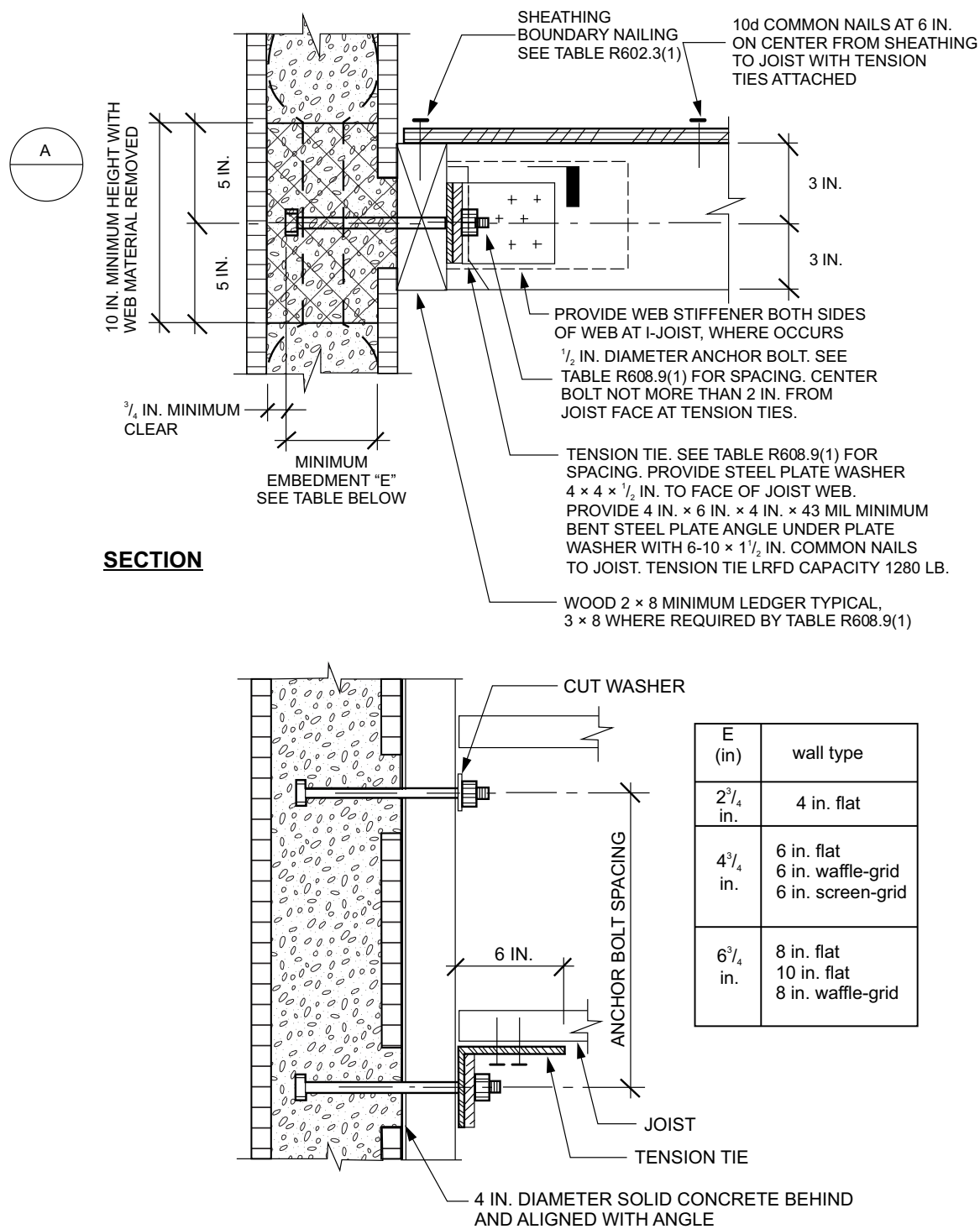
FIGURE R608.9(1)—WOOD-FRAMED FLOOR TO SIDE OF CONCRETE WALL, FRAMING PERPENDICULAR
