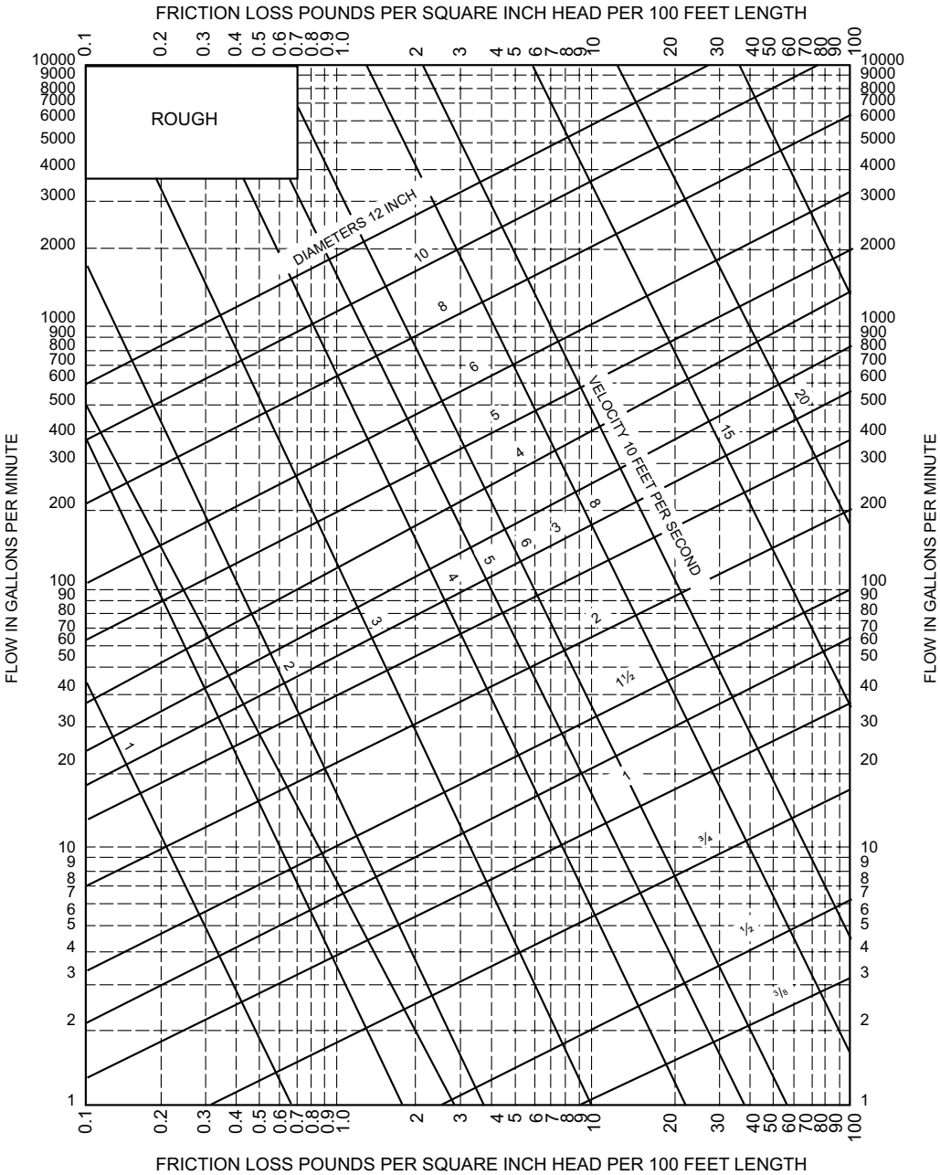
FIGURE CF103.3(7)—FRICTION LOSS IN ROUGH PIPE a
