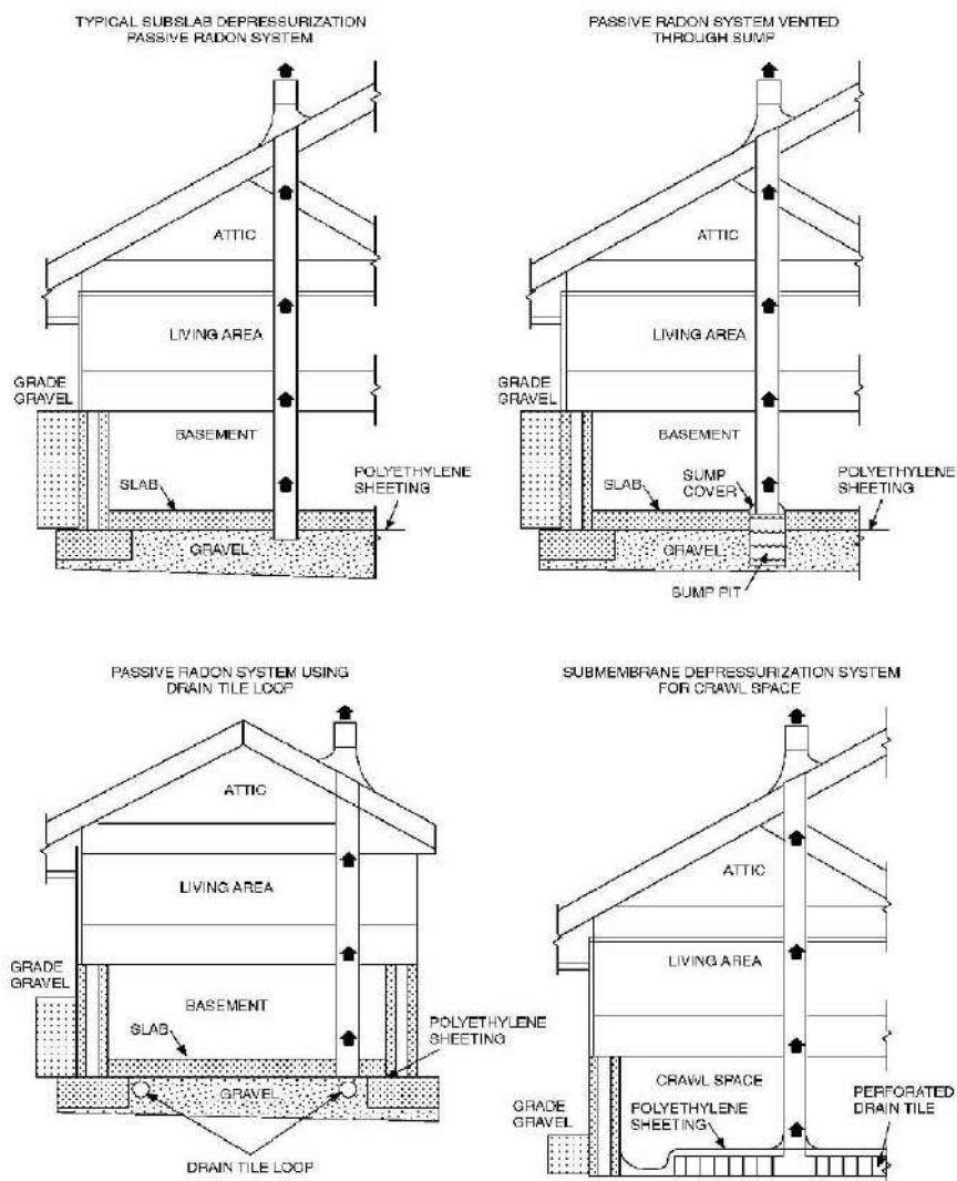
FIGURE BE103.1—RADON-RESISTANT CONSTRUCTION DETAILS FOR FOUR FOUNDATION TYPES
