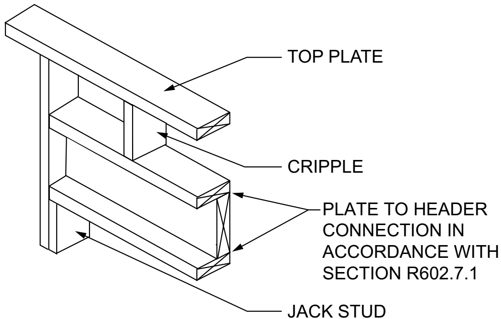
FIGURE R602.7.1(1)—SINGLE-MEMBER HEADER IN EXTERIOR BEARING WALL
