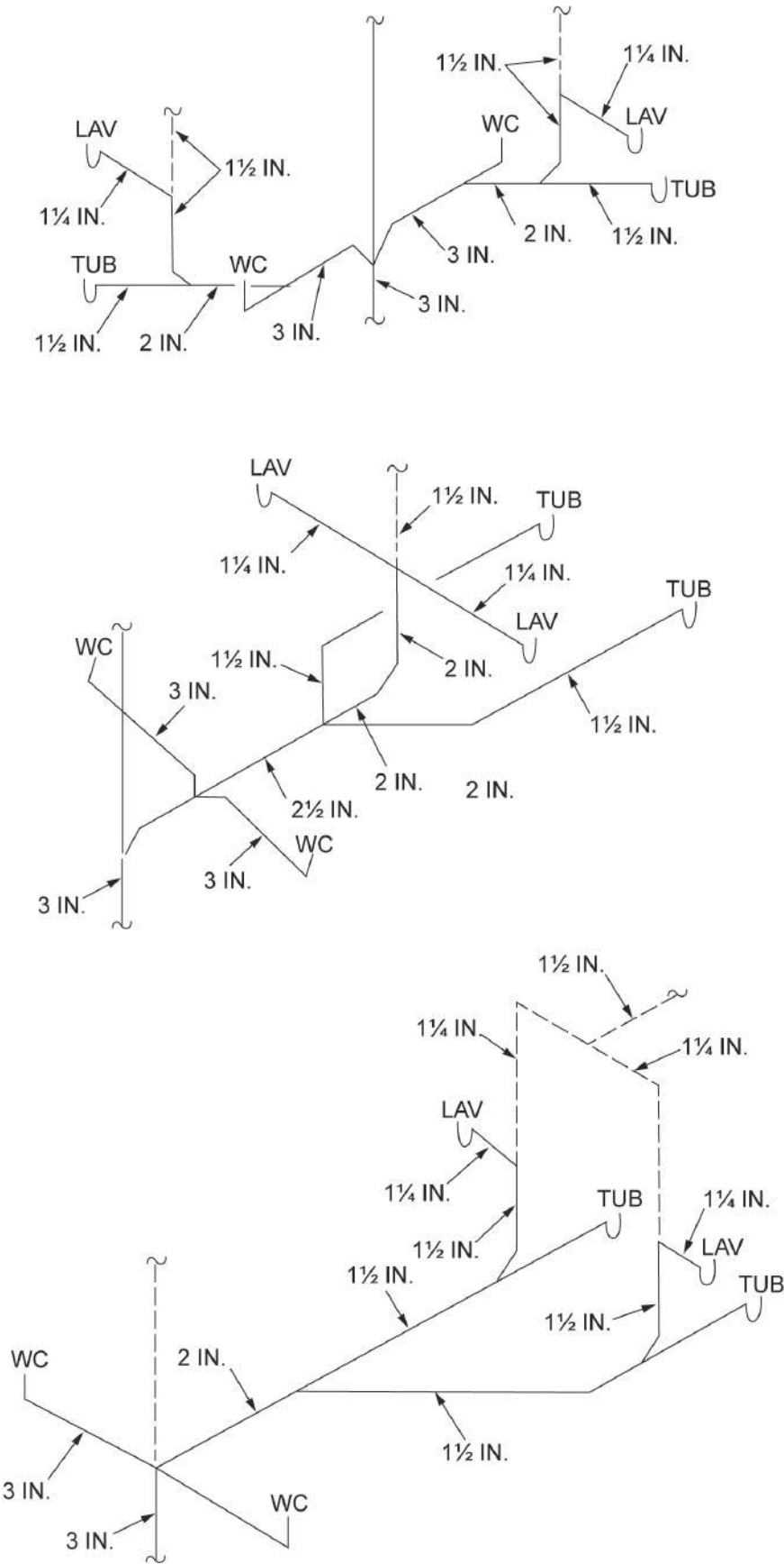
FIGURE CE101.1(2)—TYPICAL DOUBLE-BATH WET-VENT ARRANGEMENTS
