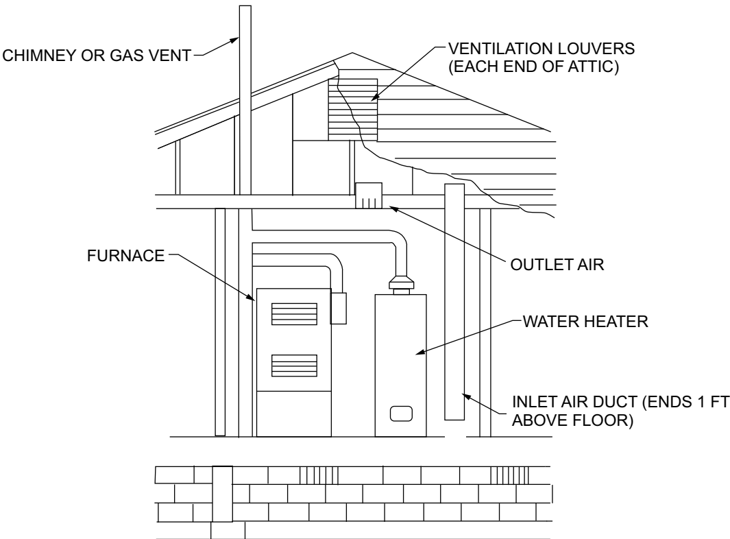
FIGURE G2407.6.1(2) [304.6.1(2)]—ALL AIR FROM OUTDOORS THROUGH VENTILATED ATTIC (see Section G2407.6.1)
