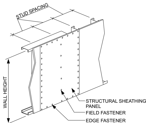
FIGURE R603.9—STRUCTURAL SHEATHING FASTENING PATTERN
