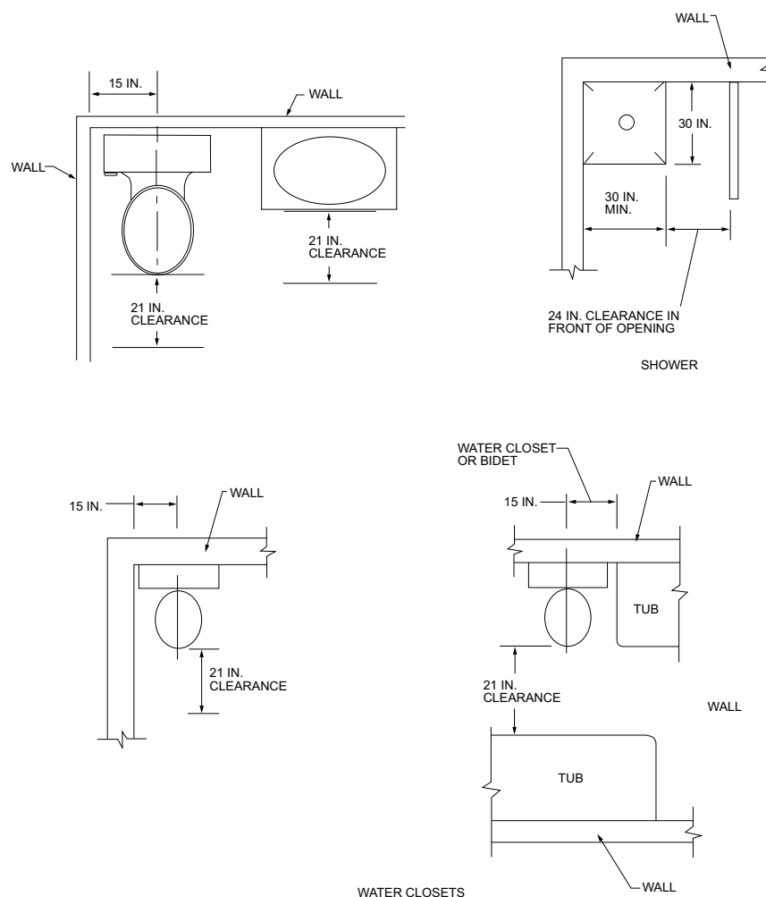
FIGURE R327.1—MINIMUM FIXTURE CLEARANCES
