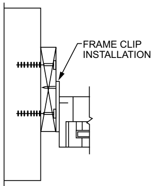
FIGURE R609.7.2(4)—FRAME CLIP
