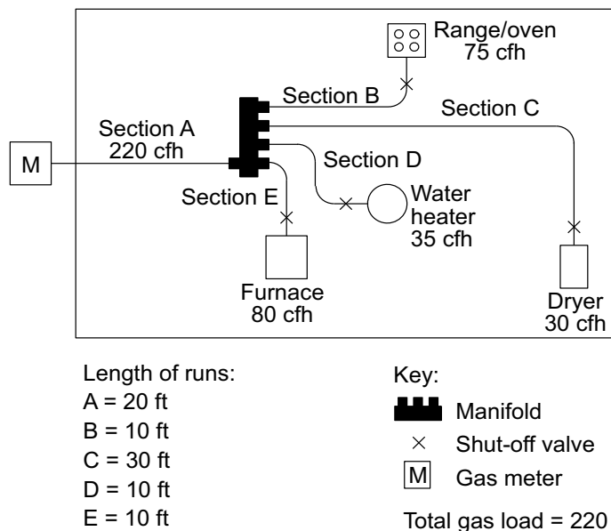
FIGURE CA106.3—PIPING PLAN SHOWING A COPPER TUBING SYSTEM
