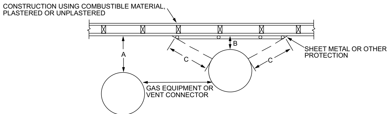
FIGURE G2409.2(1) [308.2(1)]— EXTENT OF PROTECTION NECESSARY TO REDUCE CLEARANCES FROM GAS EQUIPMENT OR VENT CONNECTORS
