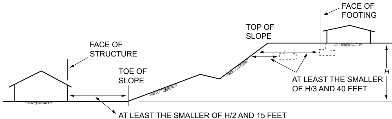
FIGURE R403.1.7.1—FOUNDATION CLEARANCE FROM SLOPES
