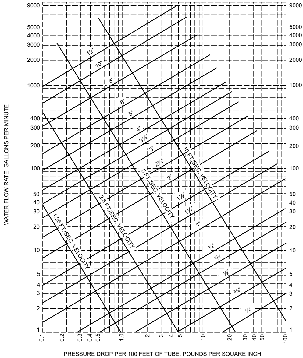
FIGURE CF103.3(2)—FRICTION LOSS IN SMOOTH PIPE 3 (TYPE K, ASTM B88 COPPER TUBING)
