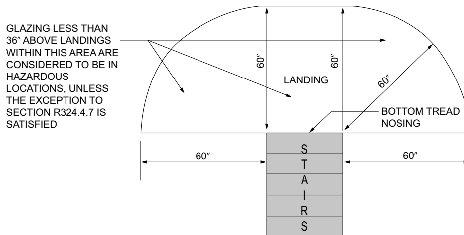
FIGURE R324.4.7—HAZARDOUS GLAZING LOCATIONS AT BOTTOM STAIR LANDINGS
