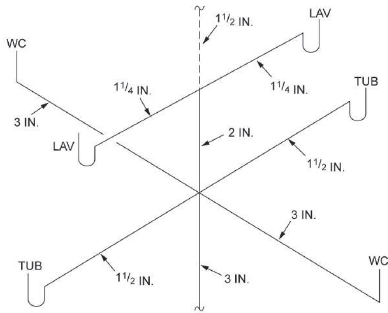
FIGURE CE101.1(4)—TYPICAL METHODS OF WET VENTING
