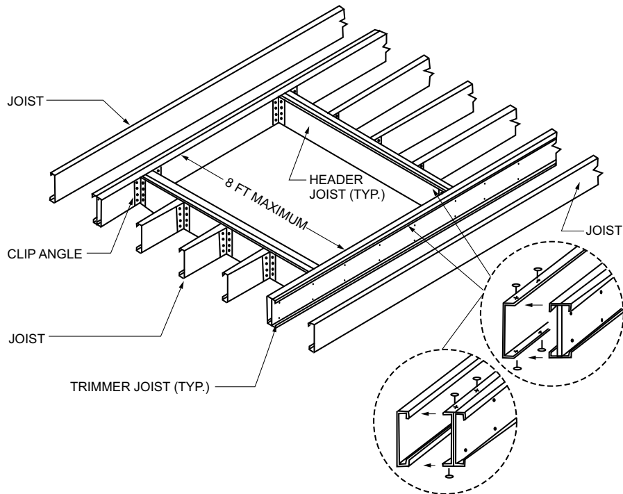
FIGURE R505.3.8(2)—COLD-FORMED STEEL FLOOR CONSTRUCTION—8-FOOT FLOOR OPENING
