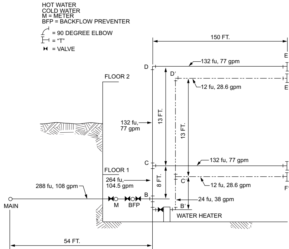
FIGURE CF103.3(1)—EXAMPLE—SIZING
