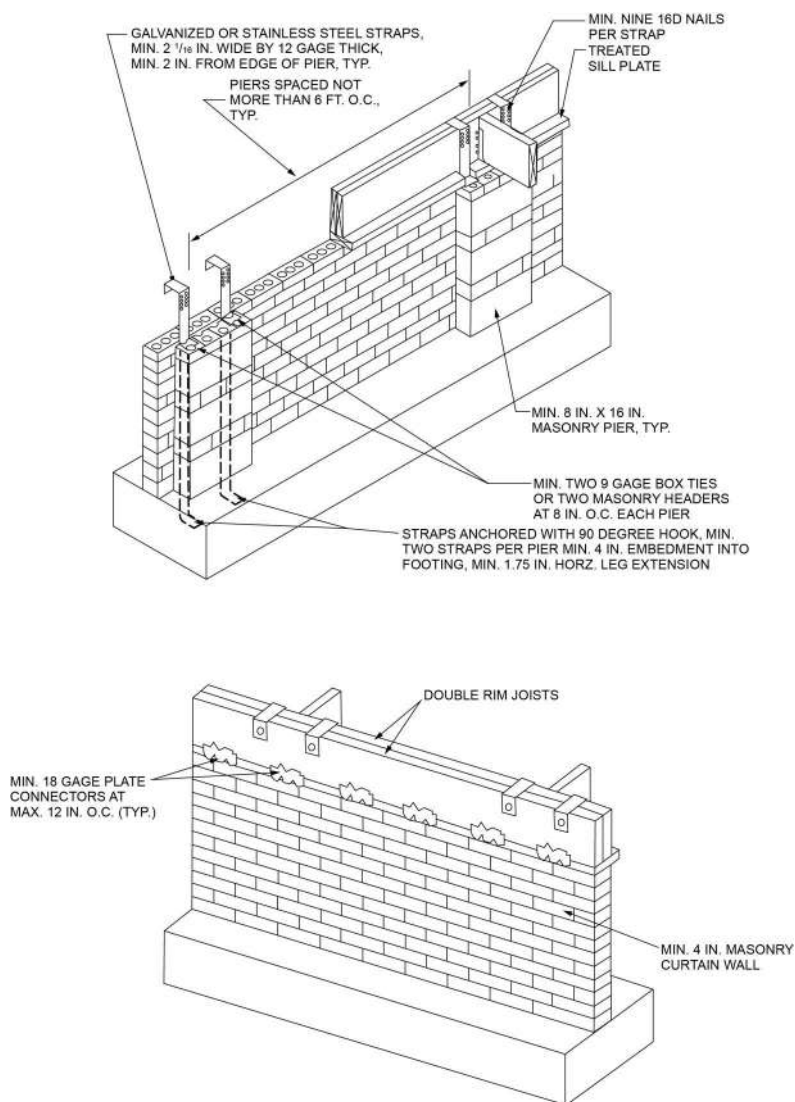
FIGURE R404.1.5.3—FOUNDATION WALL CLAY MASONRY CURTAIN WALL WITH CONCRETE MASONRY PIERS
