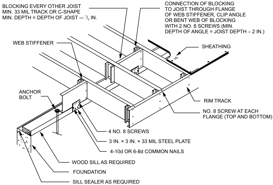
FIGURE R505.3.1(5)—CANTILEVERED FLOOR-TO-WOOD-SILL CONNECTION
