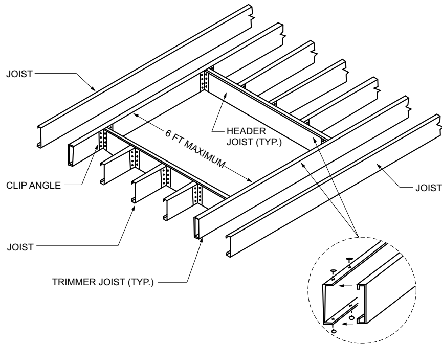
FIGURE R505.3.8(1)—COLD-FORMED STEEL FLOOR CONSTRUCTION—6-FOOT FLOOR OPENING
