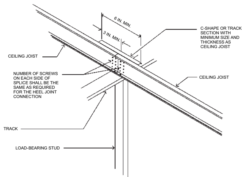
FIGURE R804.3.1.4—SPLICED CEILING JOISTS
