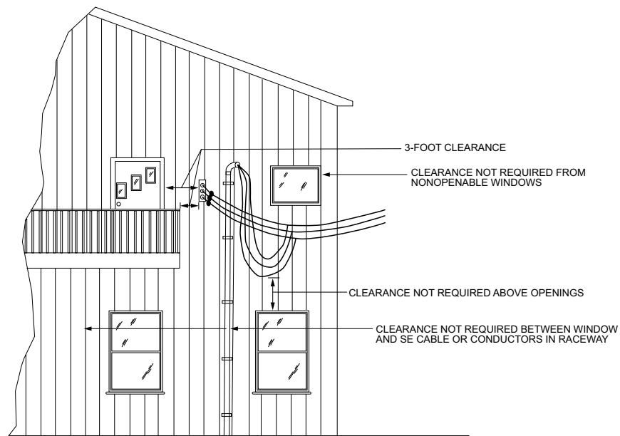
FIGURE E3604.1—CLEARANCES FROM BUILDING OPENINGS
