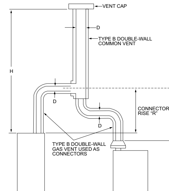
FIGURE CB102.5(1)—VENT SYSTEM SERVING TWO OR MORE APPLIANCES WITH TYPE B DOUBLE-WALL VENT AND TYPE B DOUBLE-WALL VENT CONNECTOR
