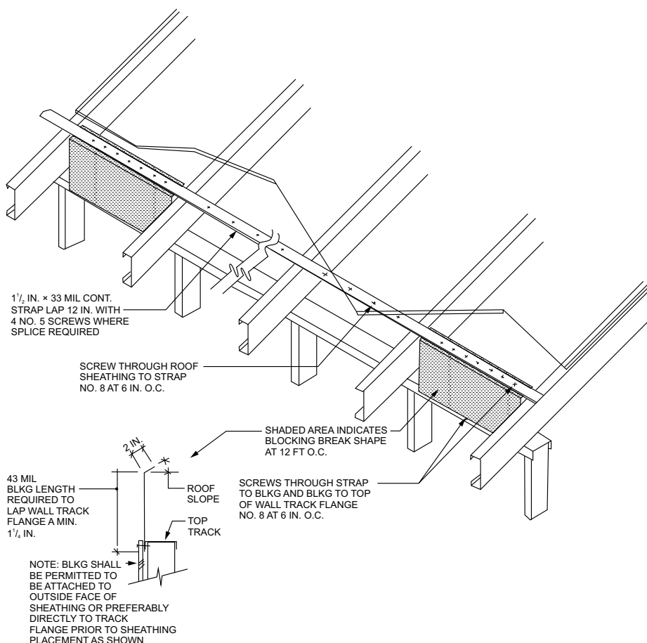
FIGURE R804.3.7.2—ROOF BLOCKING DETAIL
