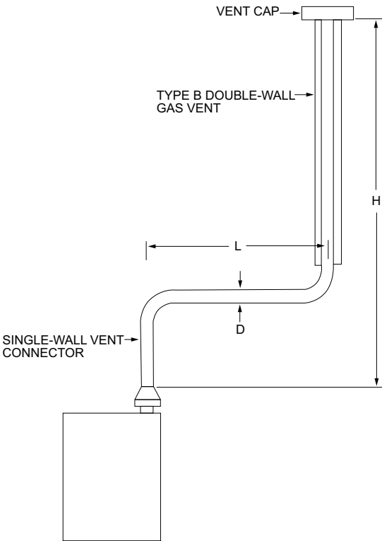
FIGURE CB101.4(2)—TYPE B DOUBLE-WALL VENT SYSTEM SERVING A SINGLE APPLIANCE WITH A SINGLE-WALL METAL VENT CONNECTOR
