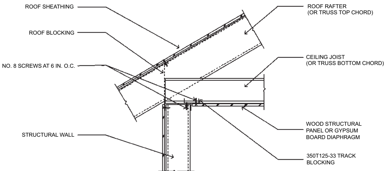
FIGURE R804.3.7.1(2)—CEILING DIAPHRAGM TO SIDEWALL DETAIL
