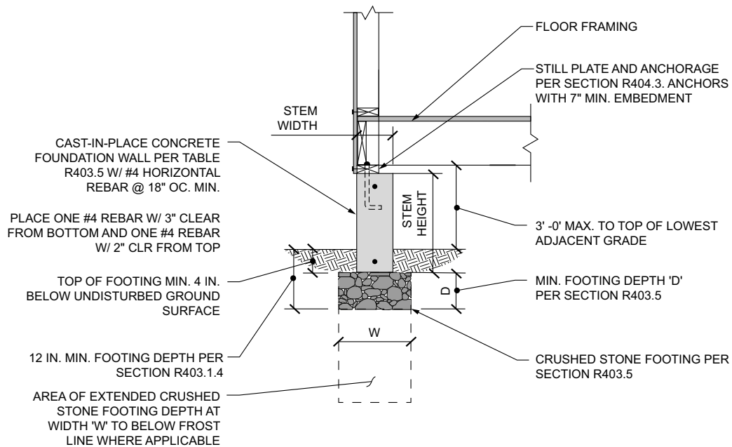
FIGURE R403.5(2)—CRUSHED STONE FOOTINGS FOR CAST-IN-PLACE CONCRETE FOUNDATIONS IN SEISMIC DESIGN CATEGORIES A, B, AND C AND WIND EXPOSURE CATEGORIES B, C, AND D: CONCRETE SLAB-ON-GROUND WITH TURNED DOWN FOUNDATION CAST-IN-PLACE CONCRETE FOUNDATION WALL WITH NO CRIPPLE WALL ABOVE
