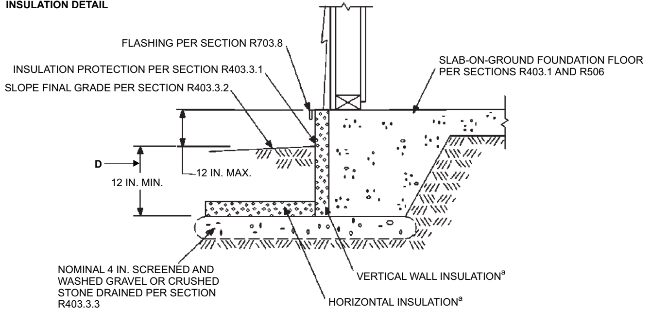
FIGURE R403.3(1)—INSULATION PLACEMENT FOR FROST-PROTECTED FOOTINGS IN HEATED BUILDINGS
