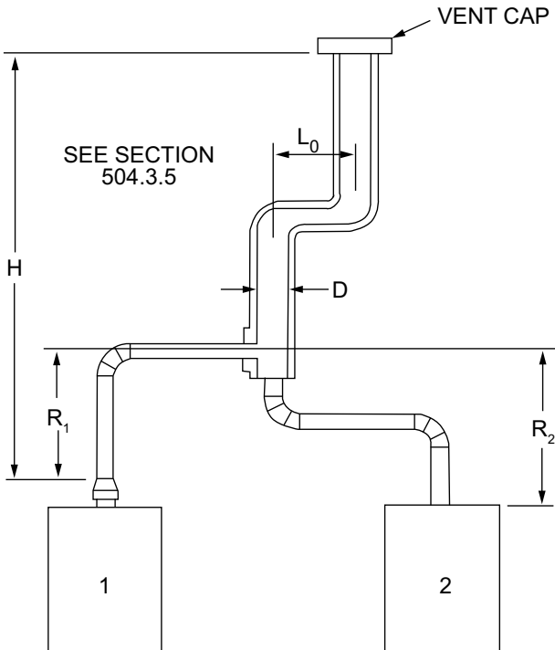
FIGURE CB102.5(5)—ASBESTOS CEMENT TYPE B OR SINGLE-WALL METAL VENT SYSTEM SERVING TWO OR MORE DRAFT HOOD-EQUIPPED APPLIANCES
