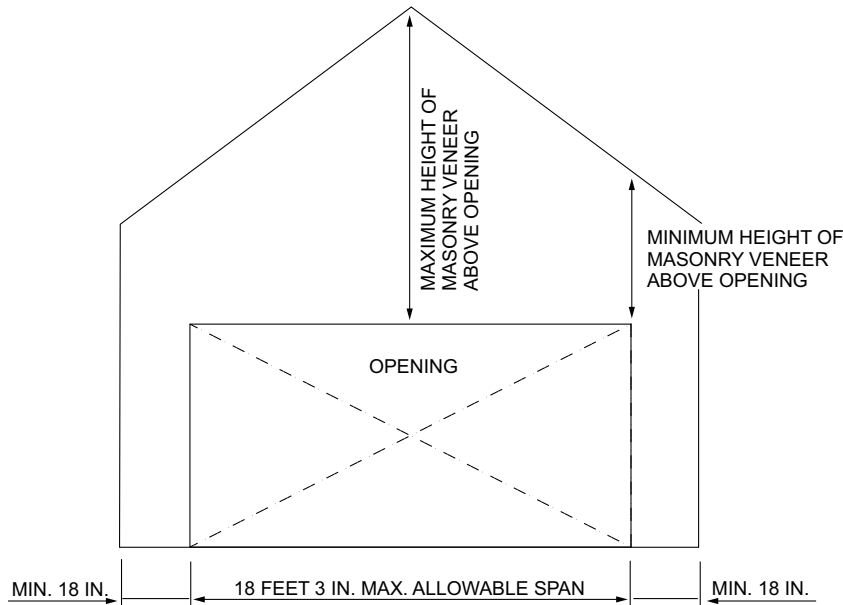
FIGURE R703.8.3.2—MASONRY VENEER OPENING
