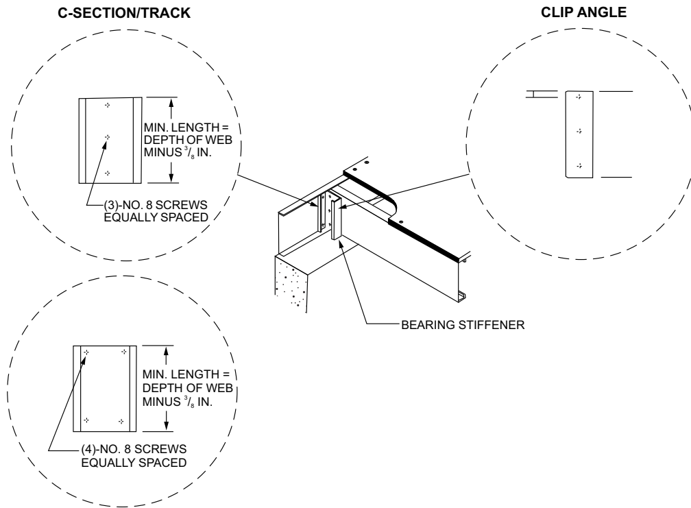
FIGURE R505.3.4(2)—BEARING STIFFENER
