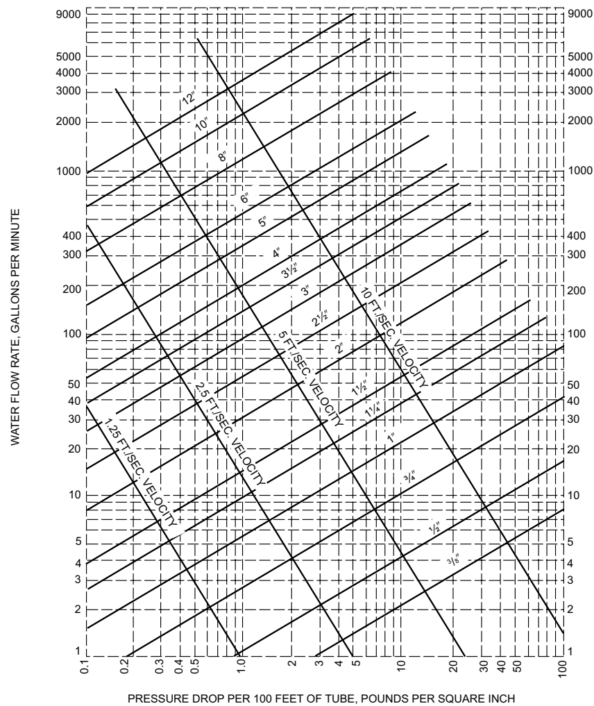
FIGURE CF103.3(4)—FRICTION LOSS IN SMOOTH PIPE 3 (TYPE M, ASTM B88 COPPER TUBING)
