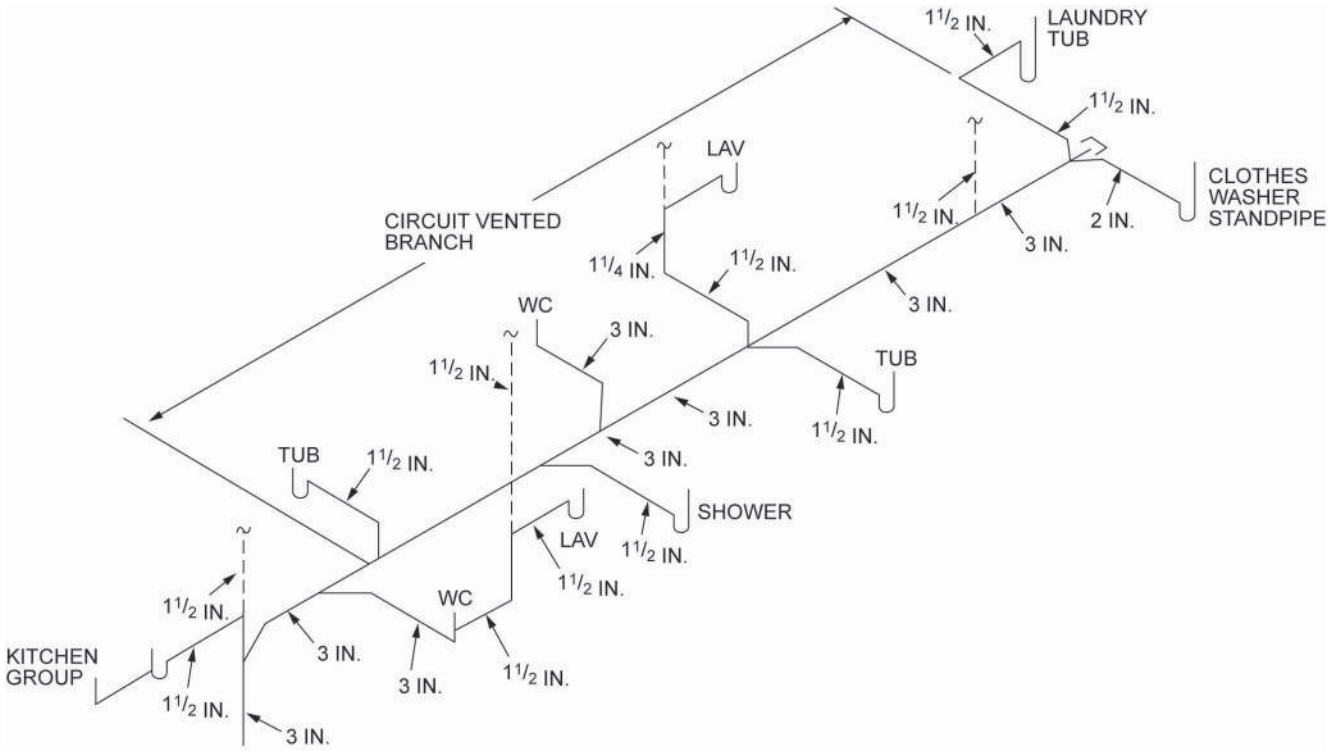
FIGURE CE101.1(7)—CIRCUIT VENT WITH ADDITIONAL NONCIRCUIT-VENTED BRANCH
