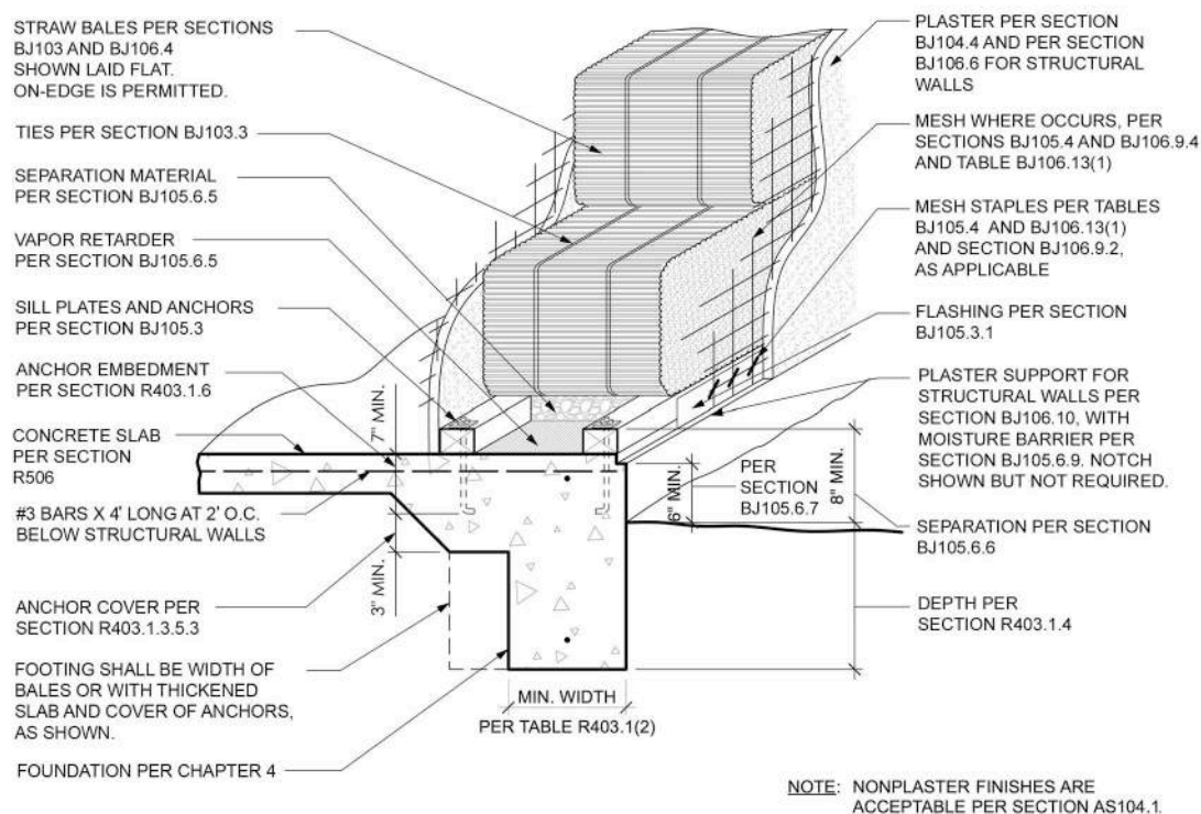
FIGURE BJ105.1(1)—TYPICAL BASE OF PLASTERED STRAWBALE WALL ON CONCRETE SLAB AND FOOTING
