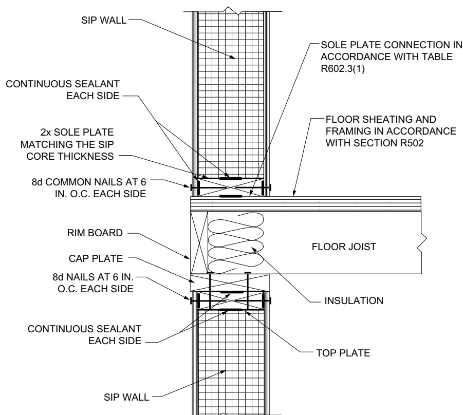
FIGURE R610.5(4)—SIP WALL-TO-WALL PLATFORM FRAME CONNECTION
