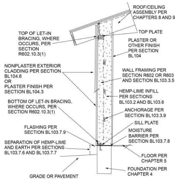
FIGURE BL103.1(3)—TYPICAL HEMP-LIME WITH EXTERIOR STUD FRAMING
