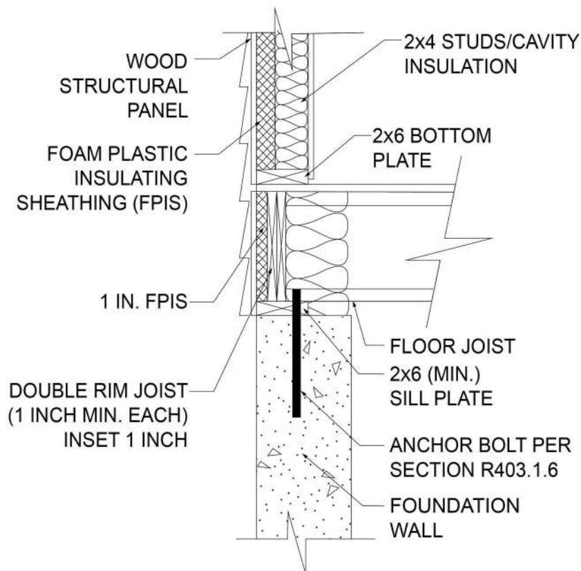
FIGURE BN102.4(2)—RIM JOIST CONSTRUCTION FOR EPW—INSET DOUBLE MEMBER
