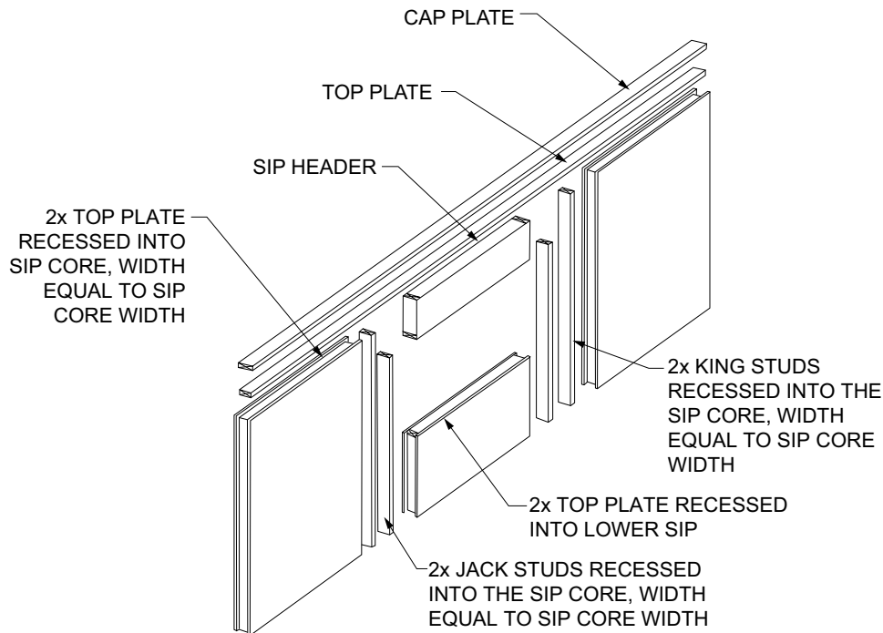
FIGURE R610.5.1—SIP WALL FRAMING CONFIGURATION
