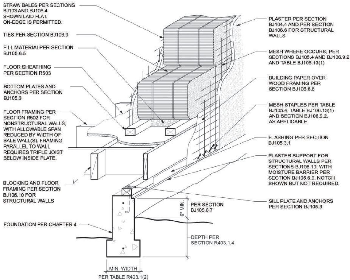
FIGURE BJ105.1(2)—TYPICAL BASE OF PLASTERED STRAWBALE WALL OVER RAISED FLOOR
