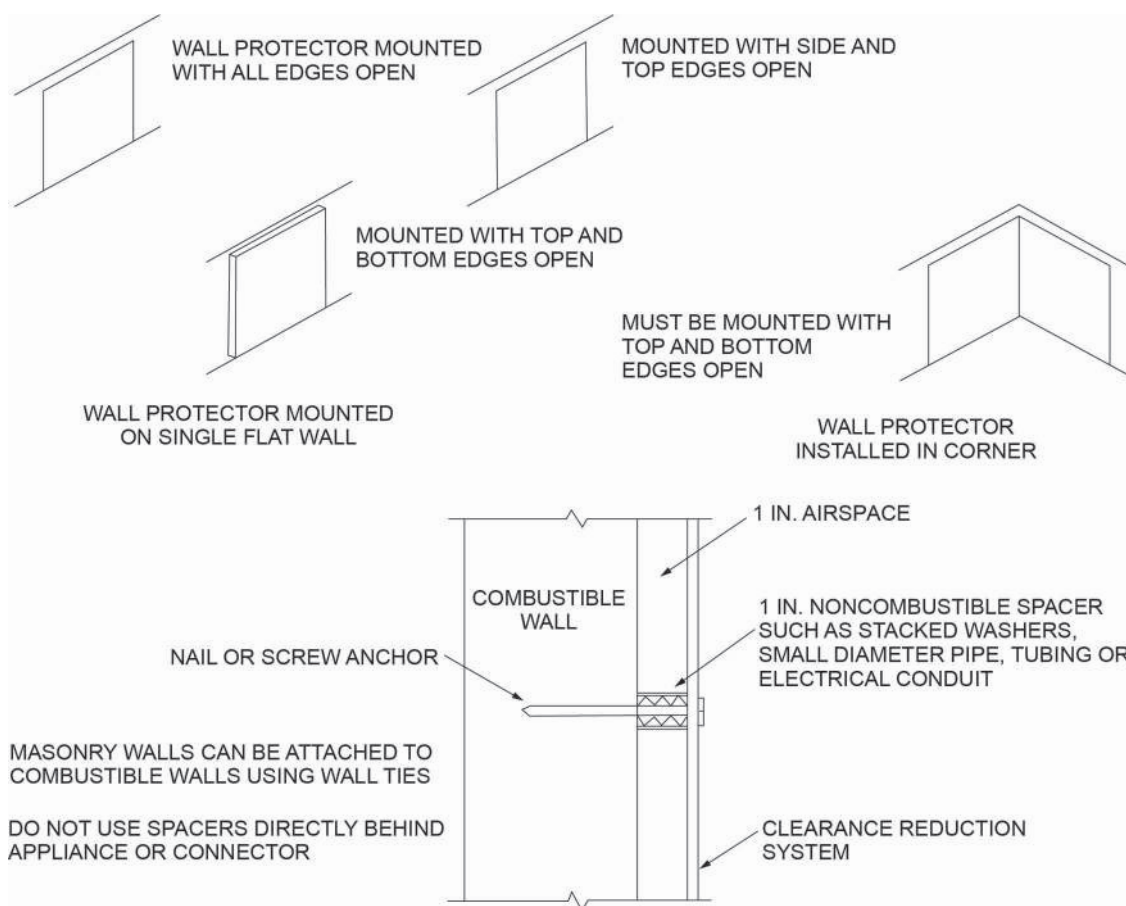
FIGURE M1306.2—WALL PROTECTOR CLEARANCE REDUCTION SYSTEM
