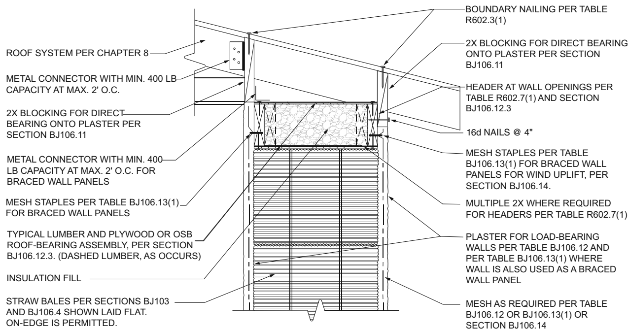
BJ105.1(3)—TYPICAL TOP OF LOAD-BEARING STRAWBALE WALL
