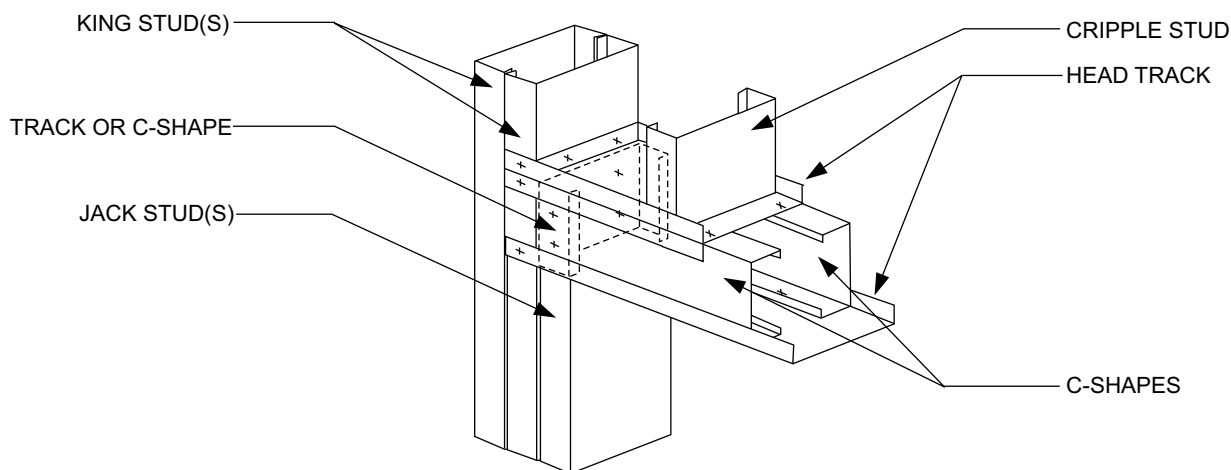
FIGURE R603.6.1(1)—BOX BEAM HEADER IN GABLE ENDWALL
