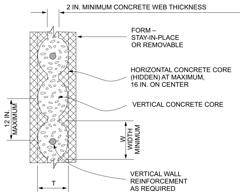
FIGURE R608.3(2)—WAFFLE-GRID WALL SYSTEM
