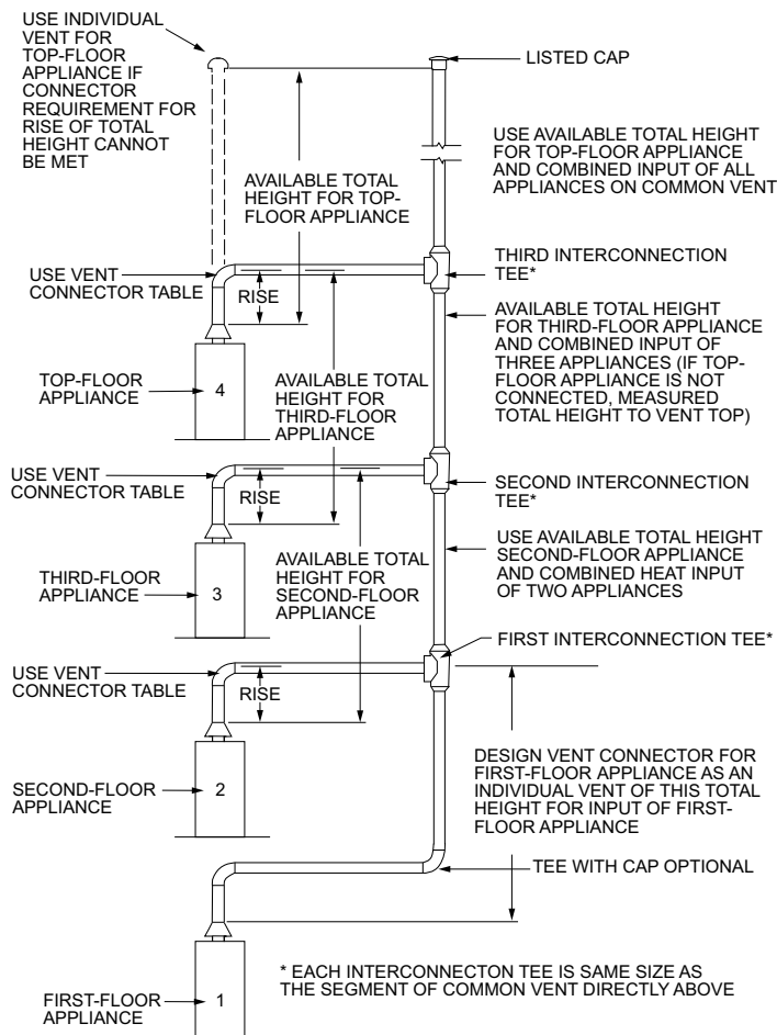
FIGURE CB102.5(9)—MULTISTORY VENT SYSTEMS
