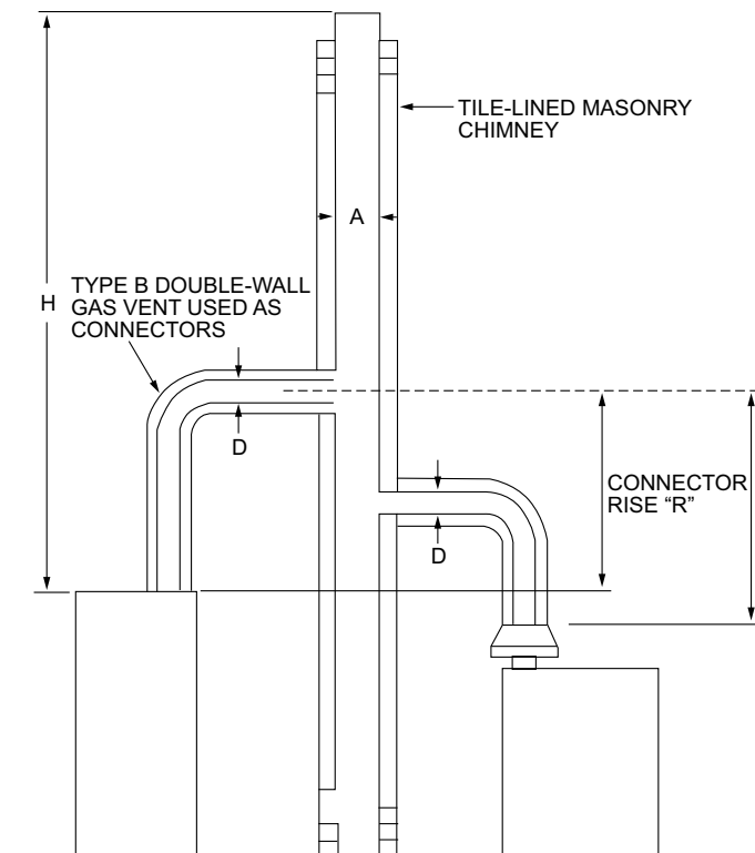
FIGURE CB102.5(3)—MASONRY CHIMNEY SERVING TWO OR MORE APPLIANCES WITH TYPE B DOUBLE-WALL VENT CONNECTOR
