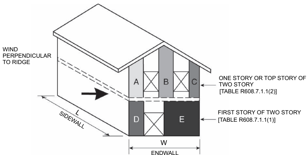
FIGURE R608.7.1.1(1)—MINIMUM SOLID WALL LENGTH
