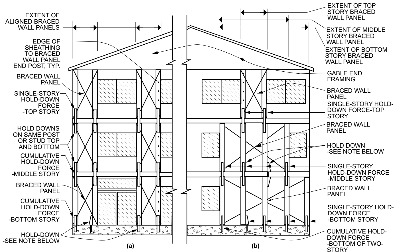
FIGURE R602.10.6.5.2—METHOD BV-WSP—WALL BRACING FOR DWELLINGS WITH STONE AND MASONRY VENEER IN SEISMIC DESIGN CATEGORIES D_0 , D_1 and D_2
