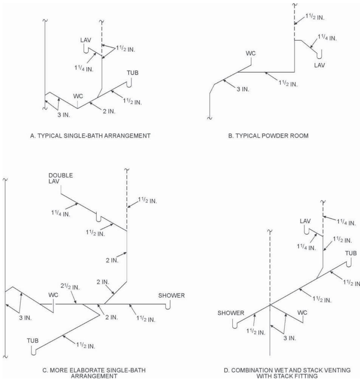
FIGURE CE101.1(1)—TYPICAL SINGLE-BATH WET-VENT ARRANGEMENTS
