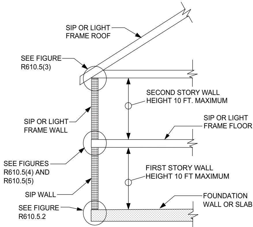
FIGURE R610.5(2)—MAXIMUM ALLOWABLE HEIGHT OF SIP WALLS
