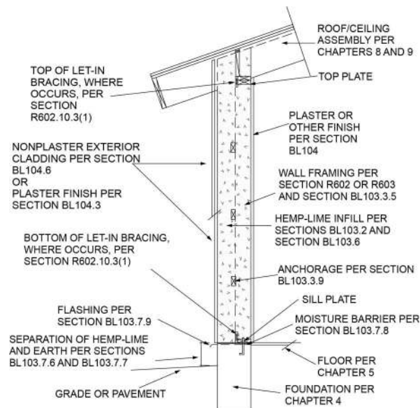
FIGURE BL103.1(1)—TYPICAL HEMP-LIME WITH INTERIOR STUD FRAMING
