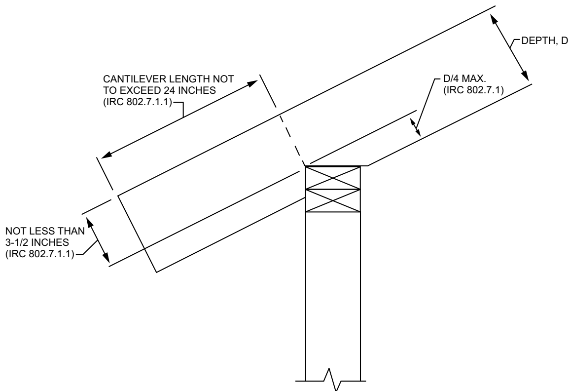
FIGURE R802.7.1.1—RAFTER NOTCH
