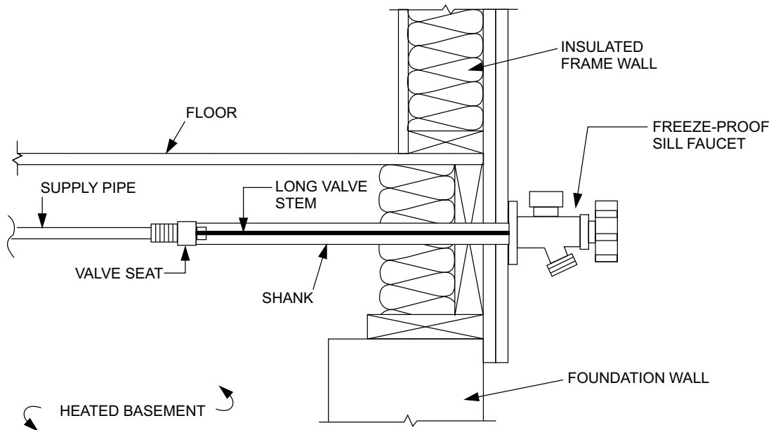
FIGURE P2903.11—TYPICAL FROSTPROOF HOSE BIBB INSTALLATION NOT REQUIRING SEPARATE VALVE
