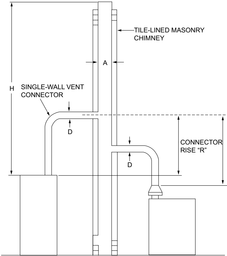
FIGURE CB102.5(4)—MASONRY CHIMNEY SERVING TWO OR MORE APPLIANCES WITH SINGLE-WALL METAL VENT CONNECTORS
