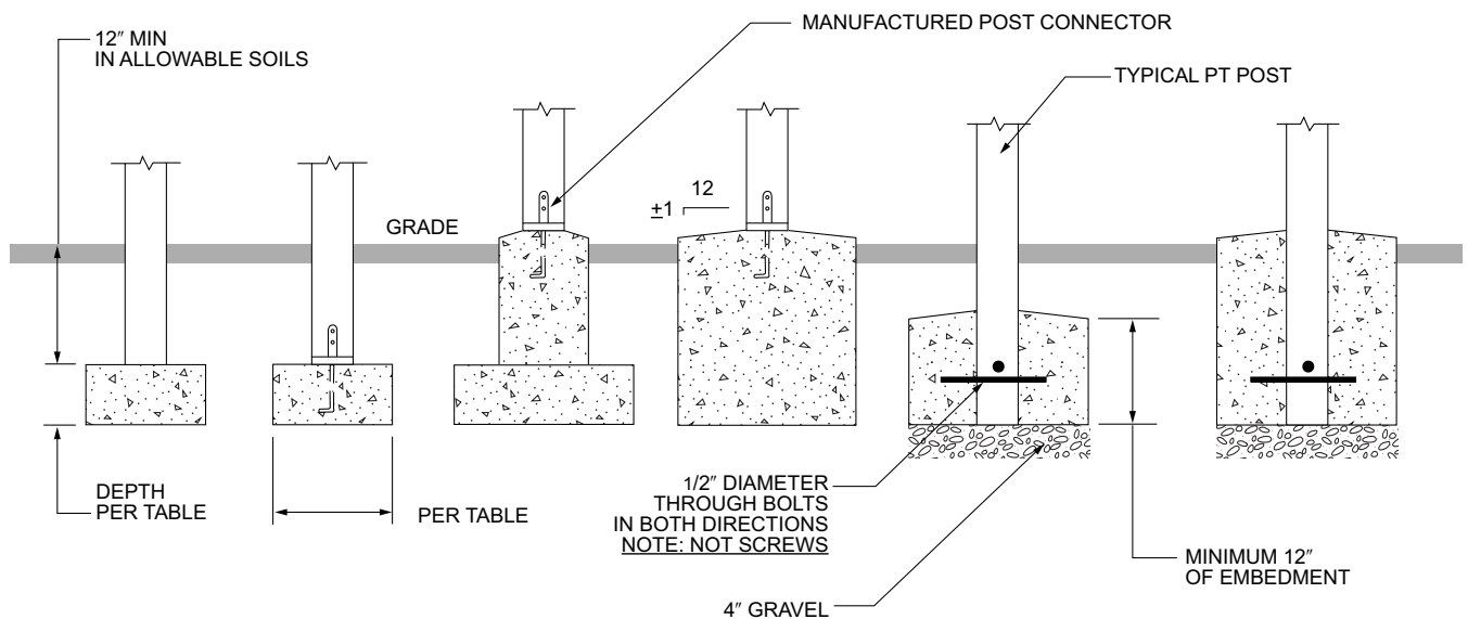
FIGURE R507.3—DECK POSTS TO DECK FOOTING CONNECTION
