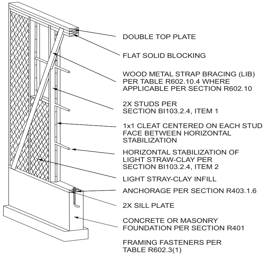
FIGURE B1103.2.4(2)—LIGHT STRAW-CLAY WALL, SINGLE STUD WIDTH
