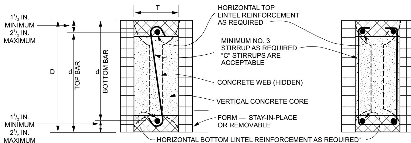
FIGURE R608.8(3)—LINTELS FOR WAFFLE-GRID WALLS
