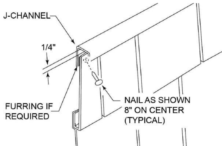
FIGURE R703.14.1.1.2 (1)—TYPICAL POLYPROPYLENE SIDING TRIM UNDER WINDOWS AND AT THE TOP OF WALLS
