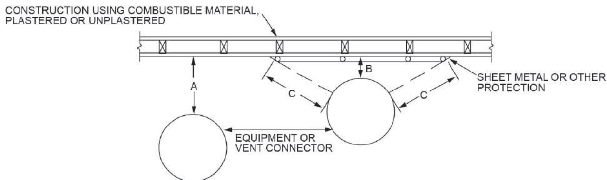
FIGURE M1306.1—REDUCED CLEARANCE DIAGRAM
