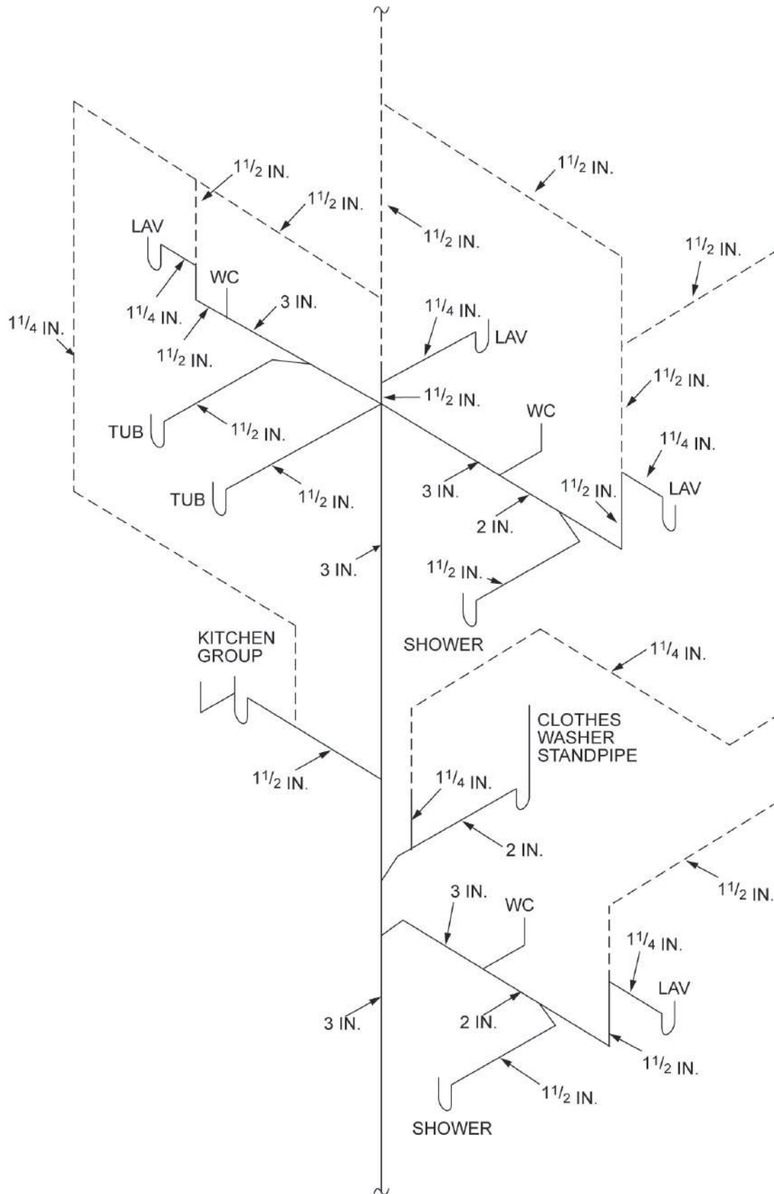
FIGURE CE101.1(5)—SINGLE-STACK SYSTEM FOR A TWO-STORY DWELLING
