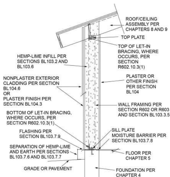
FIGURE BL103.1(2)—TYPICAL HEMP-LIME WITH CENTER STUD FRAMING
