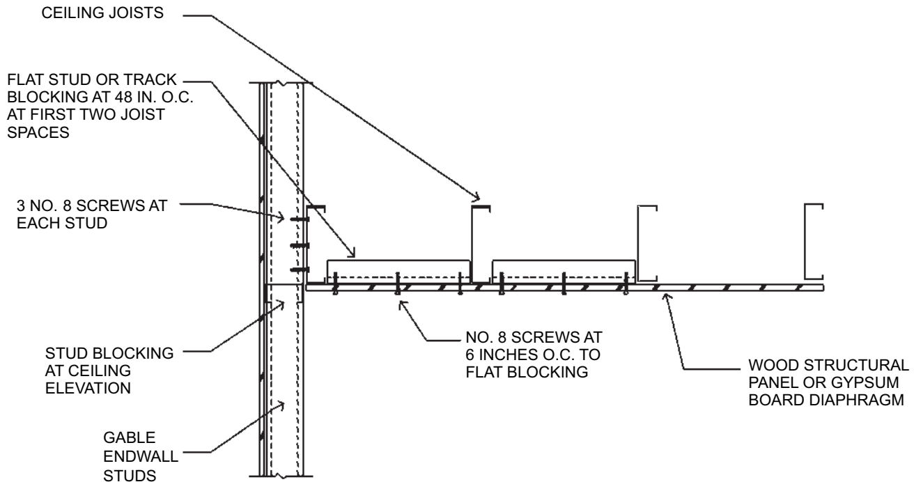
FIGURE R804.3.7.1(1)—CEILING DIAPHRAGM TO GABLE ENDWALL DETAIL
