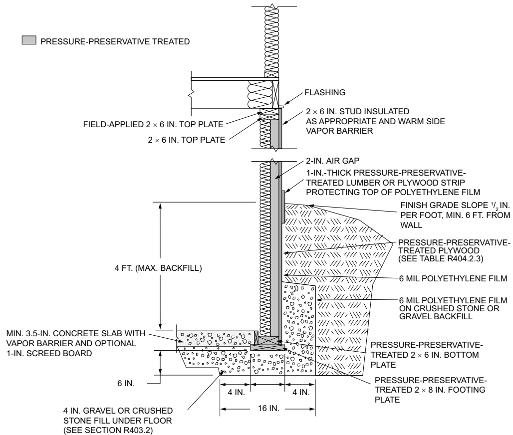
FIGURE R403.1(2)—PERMANENT WOOD FOUNDATION BASEMENT WALL SECTION
