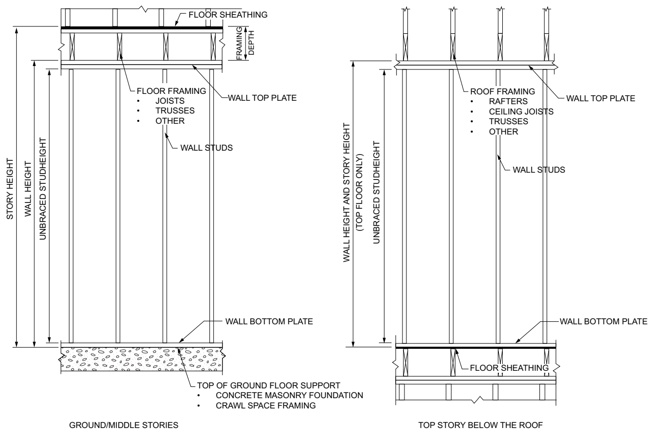
FIGURE R602.10.3.1—WALL HEIGHT FOR WOOD FRAMING
