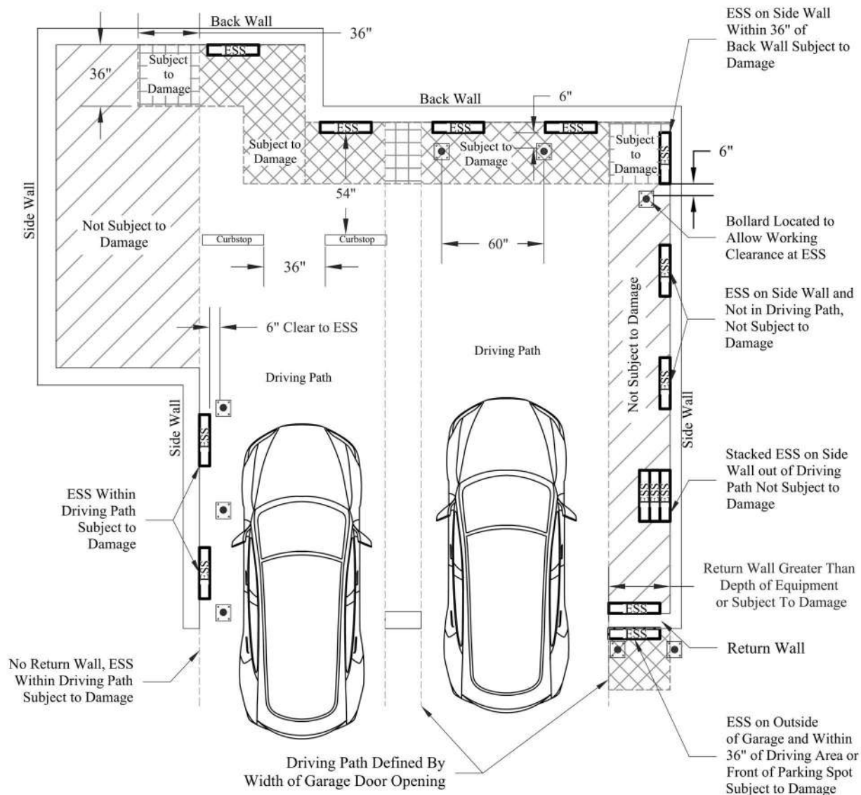
FIGURE R330.8.1—ESS VEHICLE IMPACT PROTECTION
