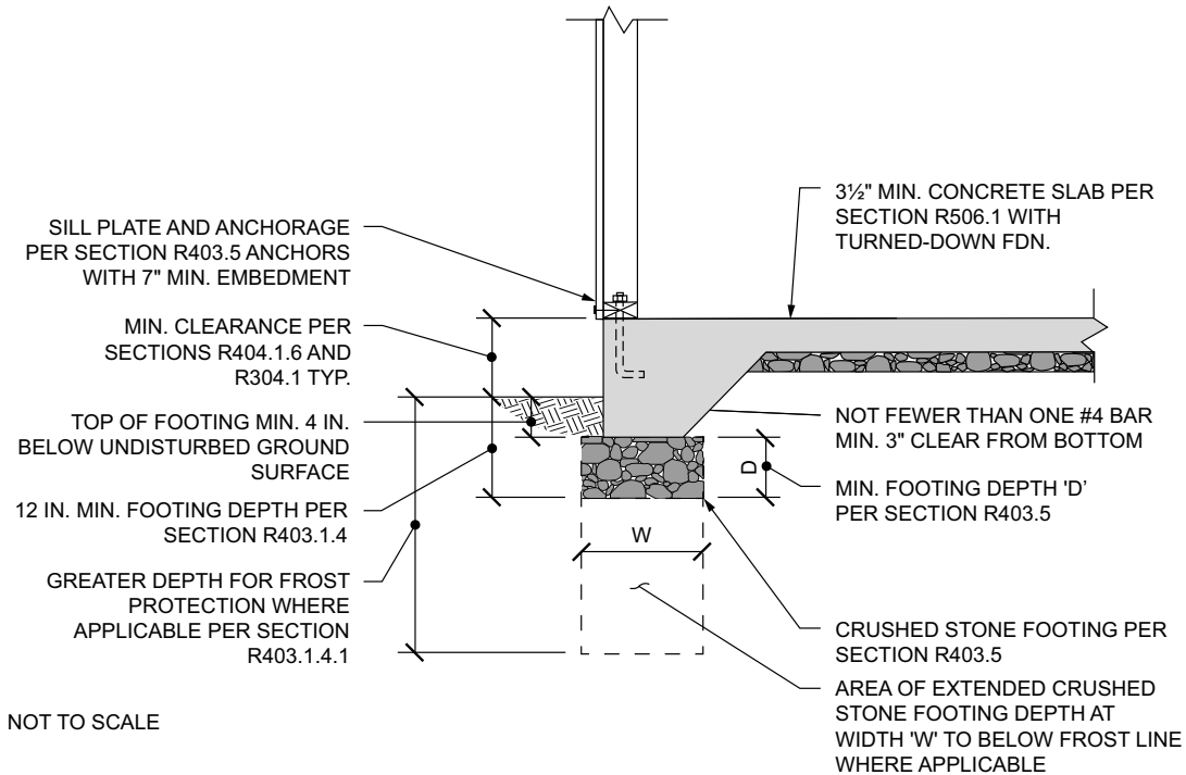
FIGURE R403.5(3)—CRUSHED STONE FOOTINGS FOR CAST-IN-PLACE CONCRETE FOUNDATIONS IN SEISMIC DESIGN CATEGORIES A, B, AND C AND WIND EXPOSURE CATEGORIES B, C, AND D: CONCRETE SLAB-ON-GROUND WITH TURNED DOWN FOUNDATION
