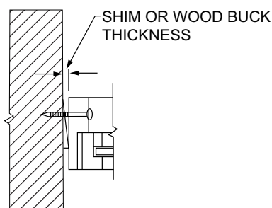
FIGURE R609.7.2(1)—THROUGH THE FRAME
