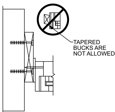
FIGURE R609.7.2(3)—THROUGH THE FRAME
