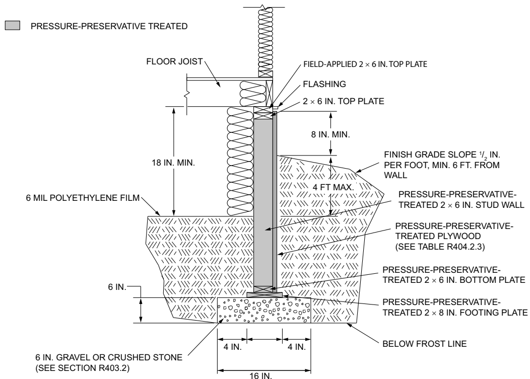
FIGURE R403.1(3)—PERMANENT WOOD FOUNDATION CRAWL SPACE SECTION
