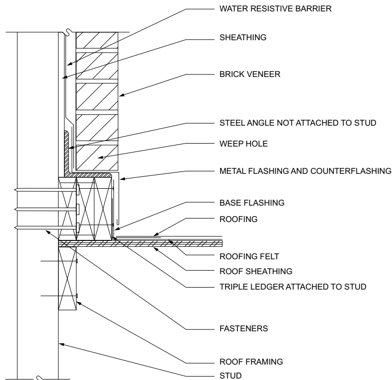
FIGURE R703.8.2.2(2)—EXTERIOR MASONRY VENEER SUPPORT BY LEDGER
