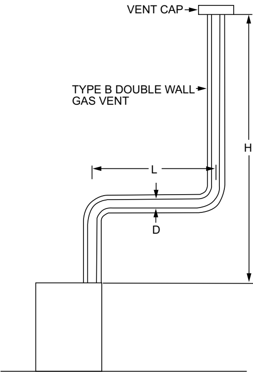
FIGURE CB101.4(1)—TYPE B DOUBLE-WALL VENT SYSTEM SERVING A SINGLE APPLIANCE WITH A TYPE B DOUBLE-WALL VENT
