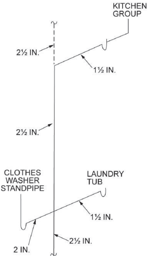
FIGURE CE101.1(6)—WASTE STACK VENTING
