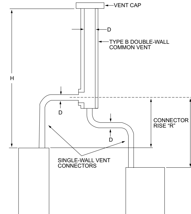
FIGURE CB102.5(2)—VENT SYSTEM SERVING TWO OR MORE APPLIANCES WITH TYPE B DOUBLE-WALL VENT AND SINGLE-WALL METAL VENT CONNECTORS
