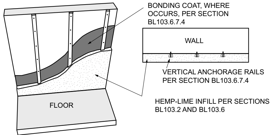
FIGURE BL103.6.7.4—TYPICAL HEMP-LIME MEDIUM LINING
