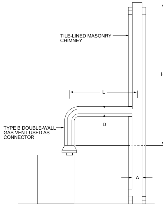
FIGURE CB101.4(3)—VENT SYSTEM SERVING A SINGLE APPLIANCE WITH A MASONRY CHIMNEY OF TYPE B DOUBLE-WALL VENT CONNECTOR
