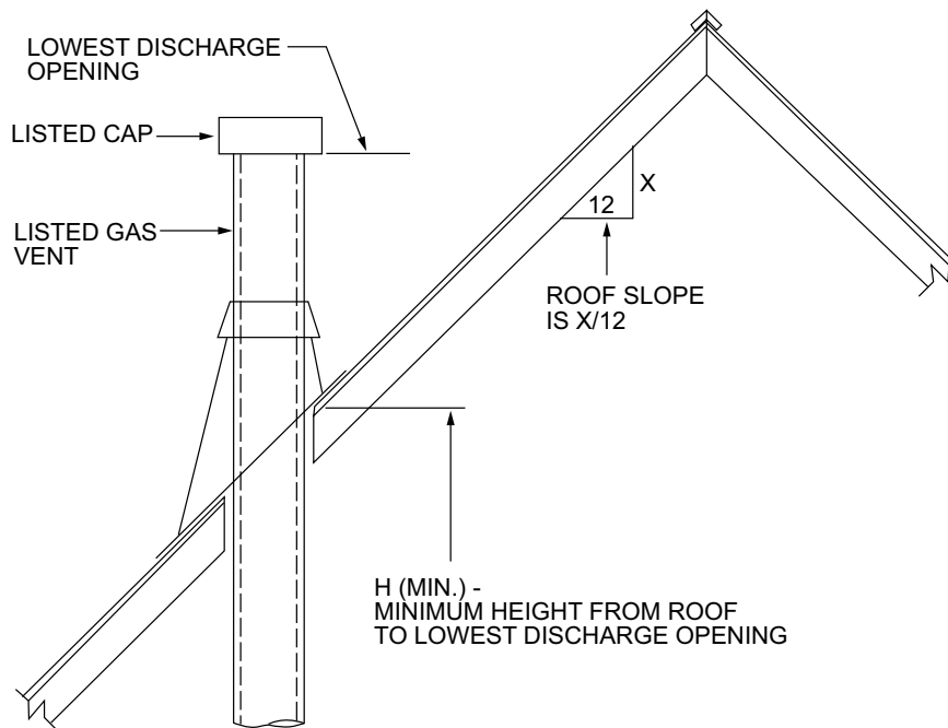
FIGURE G2427.6.4 (503.6.5)—TERMINATION LOCATIONS FOR GAS VENTS WITH LISTED CAPS 12 INCHES OR LESS IN SIZE NOT LESS THAN 8 FEET FROM A VERTICAL WALL
