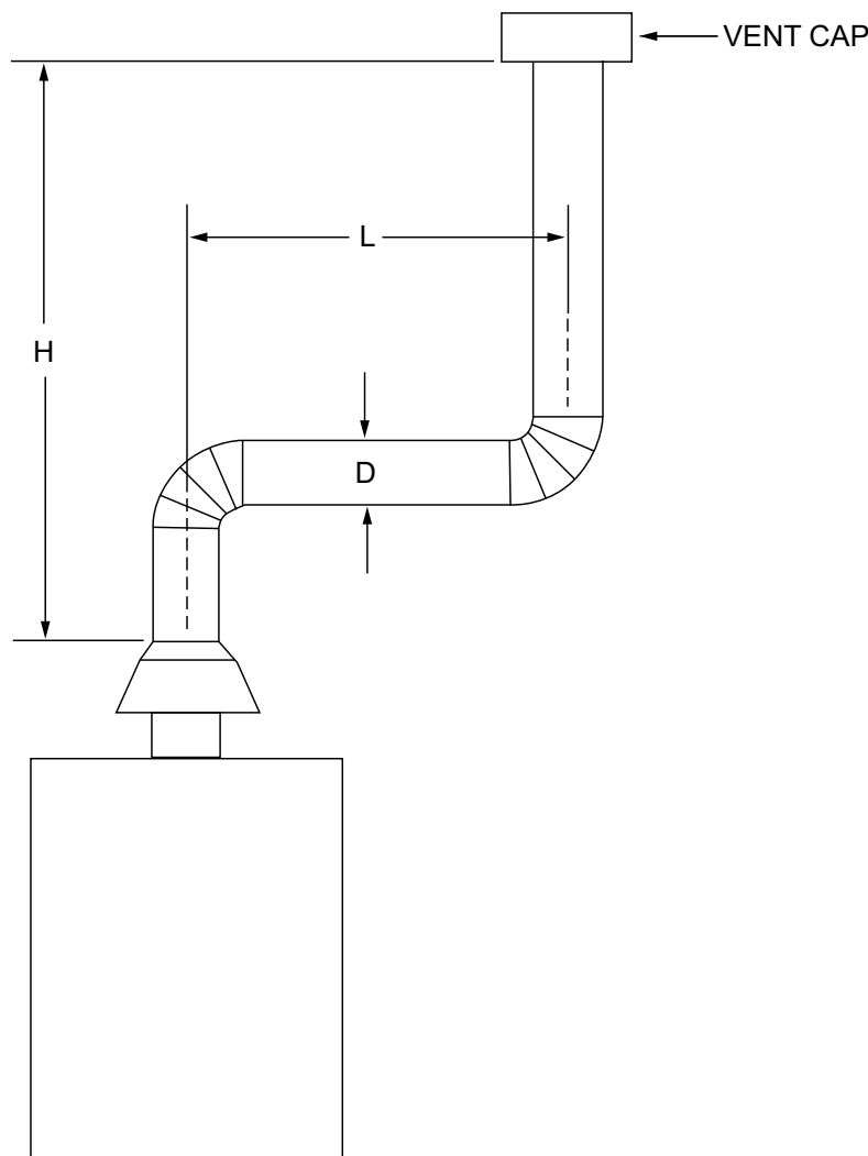
FIGURE CB101.4(5)—ASBESTOS CEMENT TYPE B OR SINGLE-WALL METAL VENT SYSTEM SERVING A SINGLE DRAFT HOOD-EQUIPPED APPLIANCE
