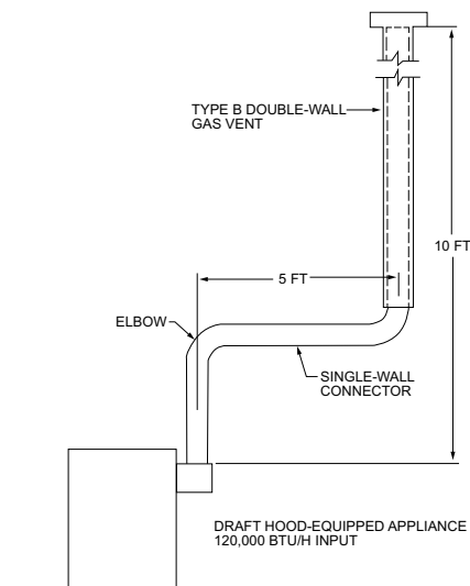
FIGURE CB101.1—EXAMPLE 1: SINGLE DRAFT HOOD-EQUIPPED APPLIANCE
