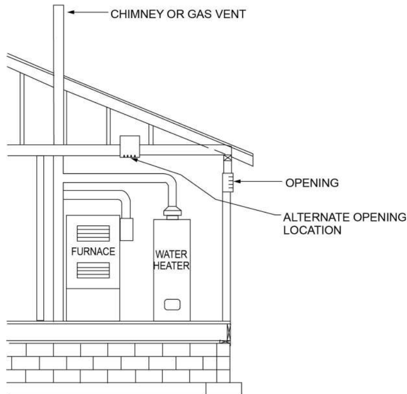
FIGURE G2407.6.2 (304.6.2)—SINGLE COMBUSTION AIR OPENING, ALL AIR FROM OUTDOORS (see Section G2407.6.2)
