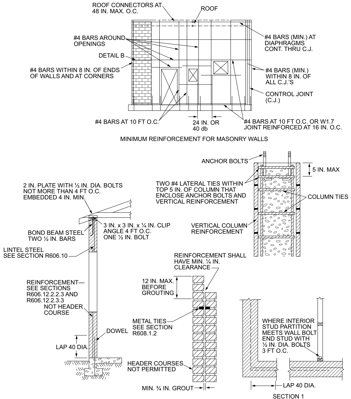
FIGURE R606.11(2)—REQUIREMENTS FOR REINFORCED GROUTED MASONRY CONSTRUCTION IN SEISMIC DESIGN CATEGORY C
