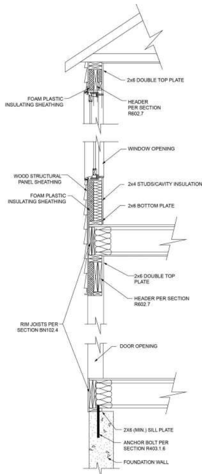
FIGURE BN102.1(1)—EXTENDED PLATE WALL (EPW) CONSTRUCTION, SECTION VIEW
