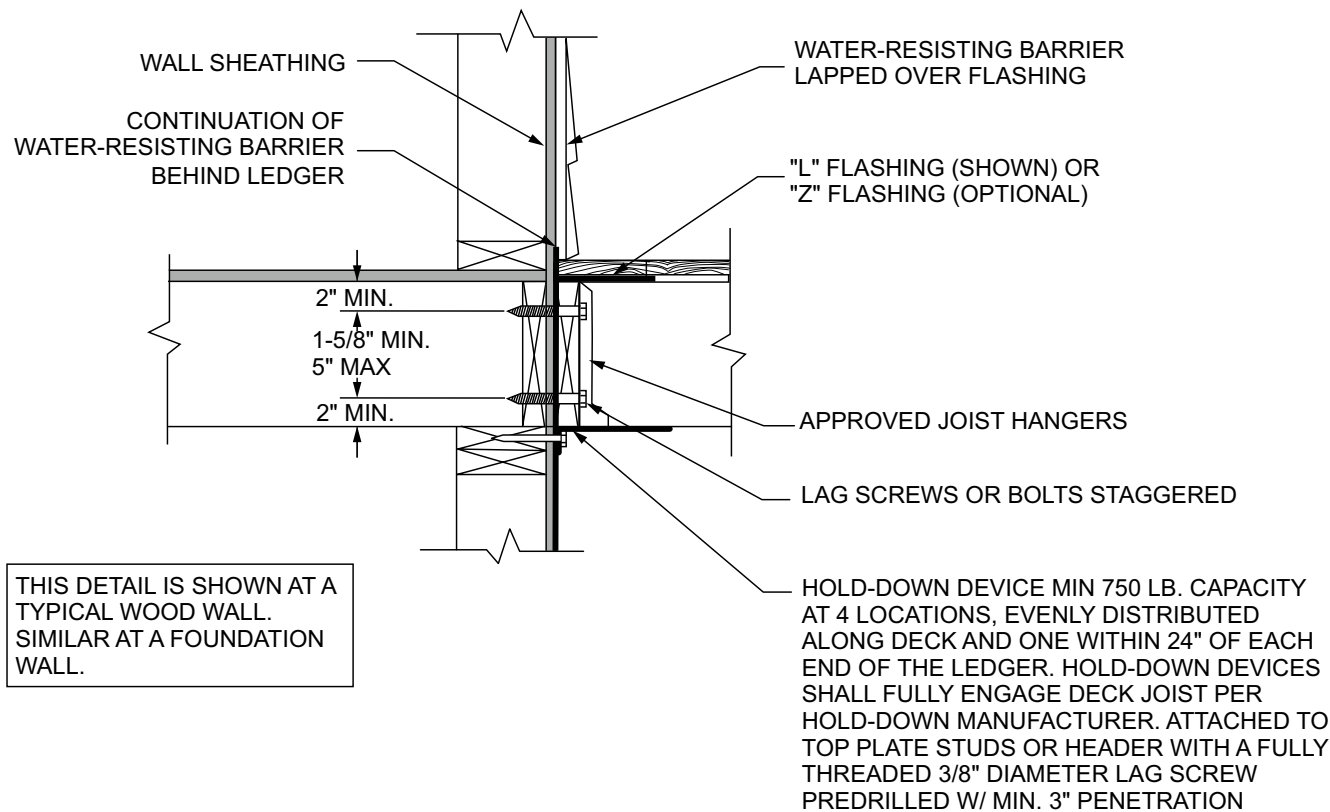
FIGURE R507.9.2(2)—DECK ATTACHMENT FOR LATERAL LOADS
