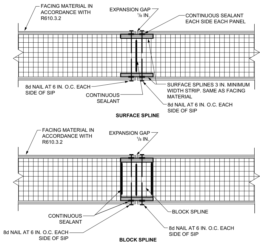
FIGURE R610.8—TYPICAL SIP WALL PANEL-TO-PANEL CONNECTION DETAILS
