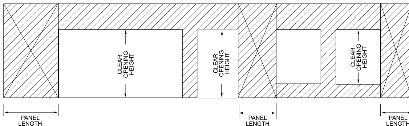
FIGURE R602.10.5—BRACED WALL PANELS WITH CONTINUOUS SHEATHING
