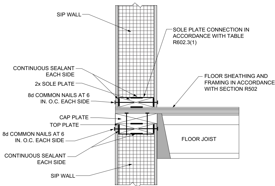
FIGURE R610.5(5)—SIP WALL-TO-WALL HANGING FLOOR FRAME CONNECTION (I-Joist floor shown for illustration only)
