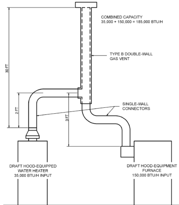
FIGURE CB102.1—EXAMPLE 4: COMMON VENTING TWO DRAFT HOOD-EQUIPPED APPLIANCES
