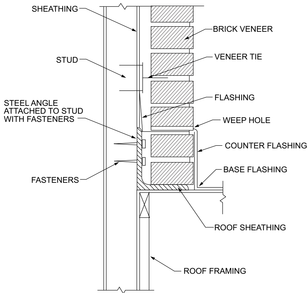
FIGURE R703.8.2.1—EXTERIOR MASONRY VENEER SUPPORT BY STEEL ANGLES
