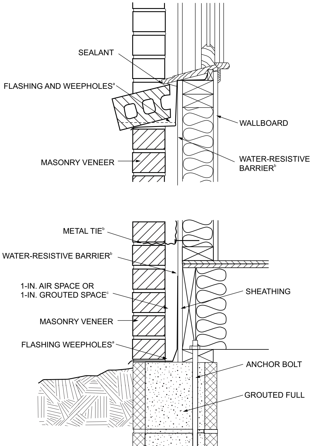
FIGURE R703.8(1)—TYPICAL MASONRY VENEER WALL DETAILS d
