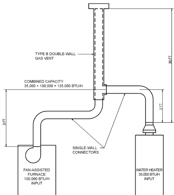
FIGURE CB102.2—EXAMPLE 5a: COMMON VENTING A DRAFT HOOD WITH A FAN-ASSISTED FURNACE INTO A TYPE B DOUBLE-WALL COMMON VENT
