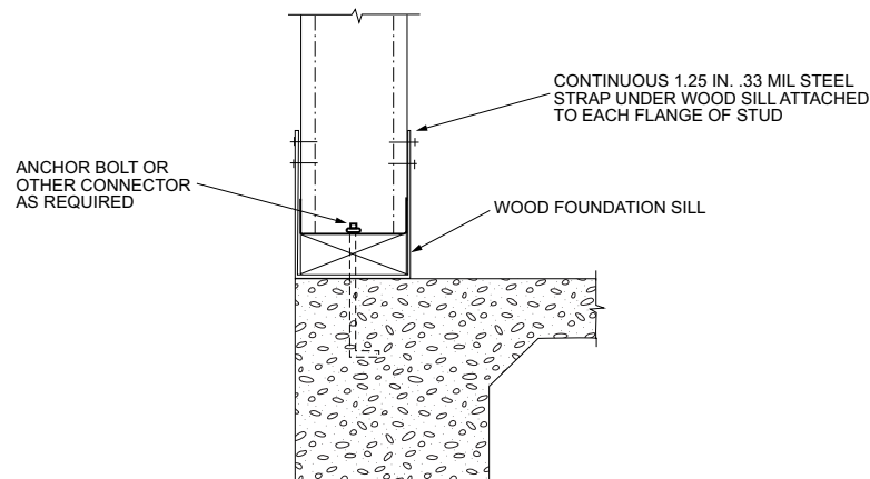
FIGURE R603.3.1(4)—WIND UPLIFT CONNECTOR
