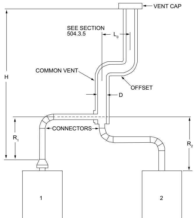
FIGURE CB102.5(7)—USE OF OFFSET COMMON VENTS WITH SINGLE-WALL METAL VENT CONNECTORS
