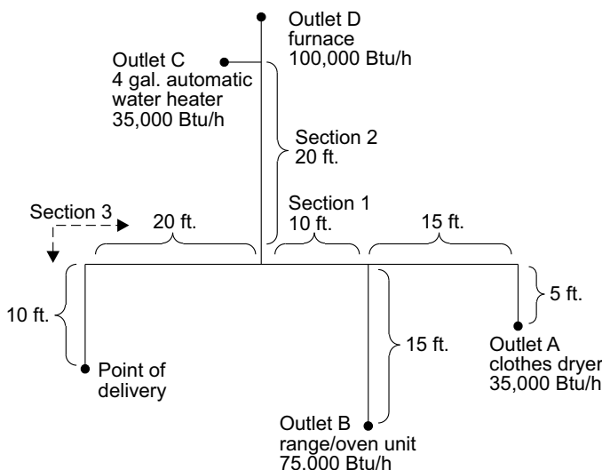
FIGURE CA106.1—PIPING PLAN SHOWING A STEEL PIPING SYSTEM
