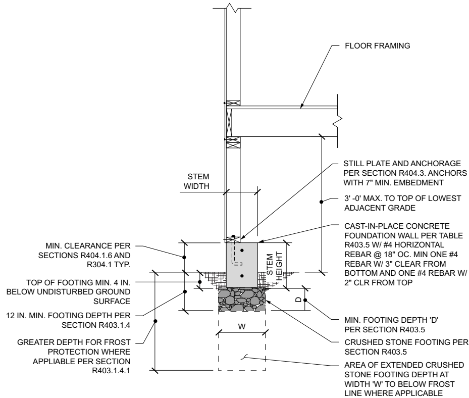
FIGURE R403.5(1)—CRUSHED STONE FOOTINGS FOR CAST-IN-PLACE CONCRETE FOUNDATIONS IN SEISMIC DESIGN CATEGORIES A, B, AND C AND WIND EXPOSURE CATEGORIES B, C, AND D: CAST-IN-PLACE CONCRETE FOUNDATION WALL WITH WOOD CRIPPLE WALL
