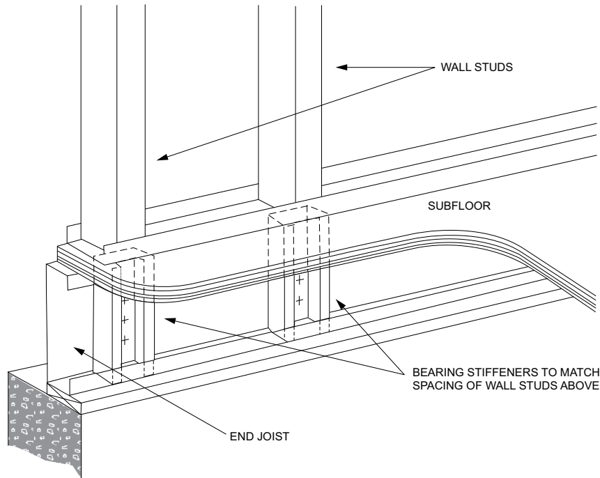
FIGURE R505.3.1(9)—BEARING STIFFENERS FOR END JOISTS
