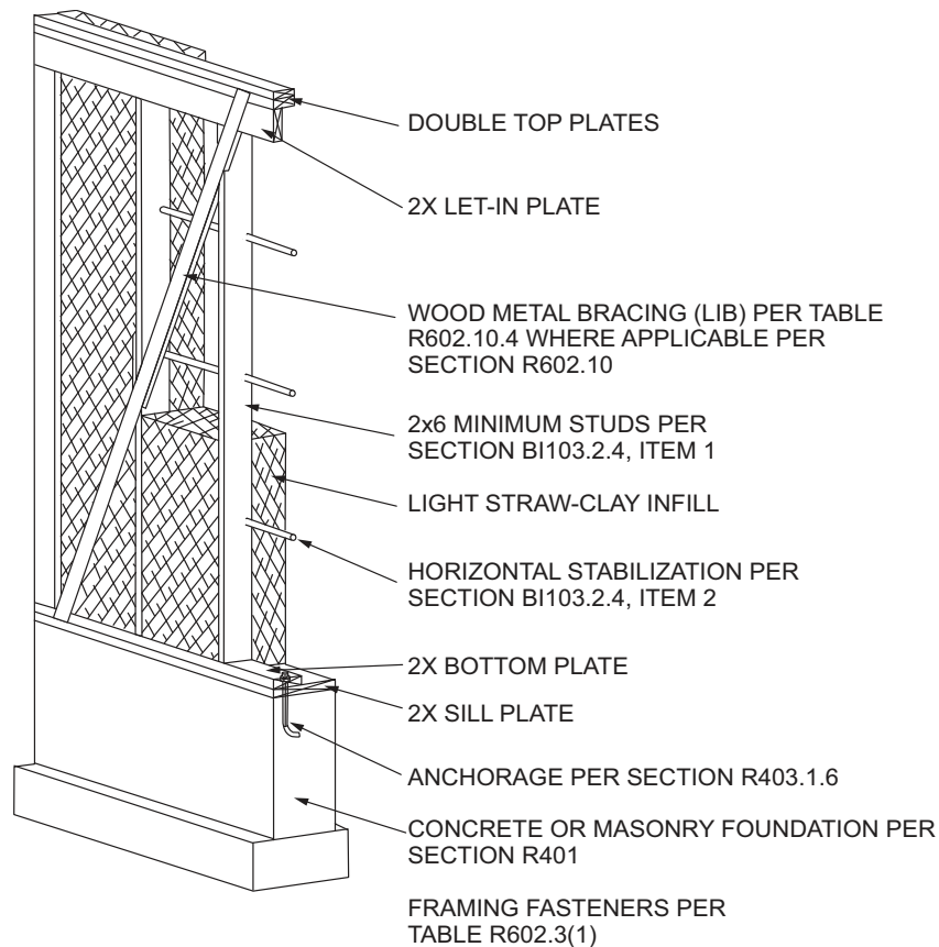
FIGURE B1103.2.4(3)—LIGHT STRAW-CLAY WALL WITH BLIND STUDS
