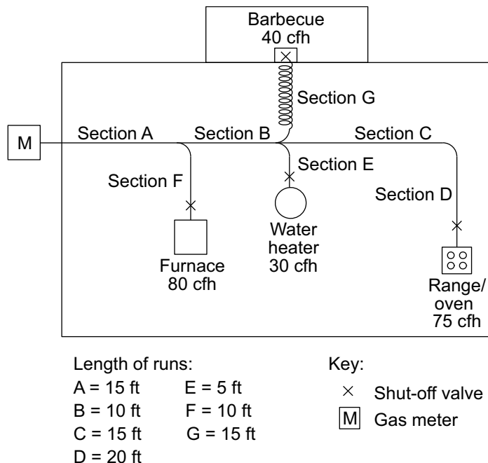
FIGURE CA106.4—PIPING PLAN SHOWING A MODIFICATION TO EXISTING PIPING SYSTEM
