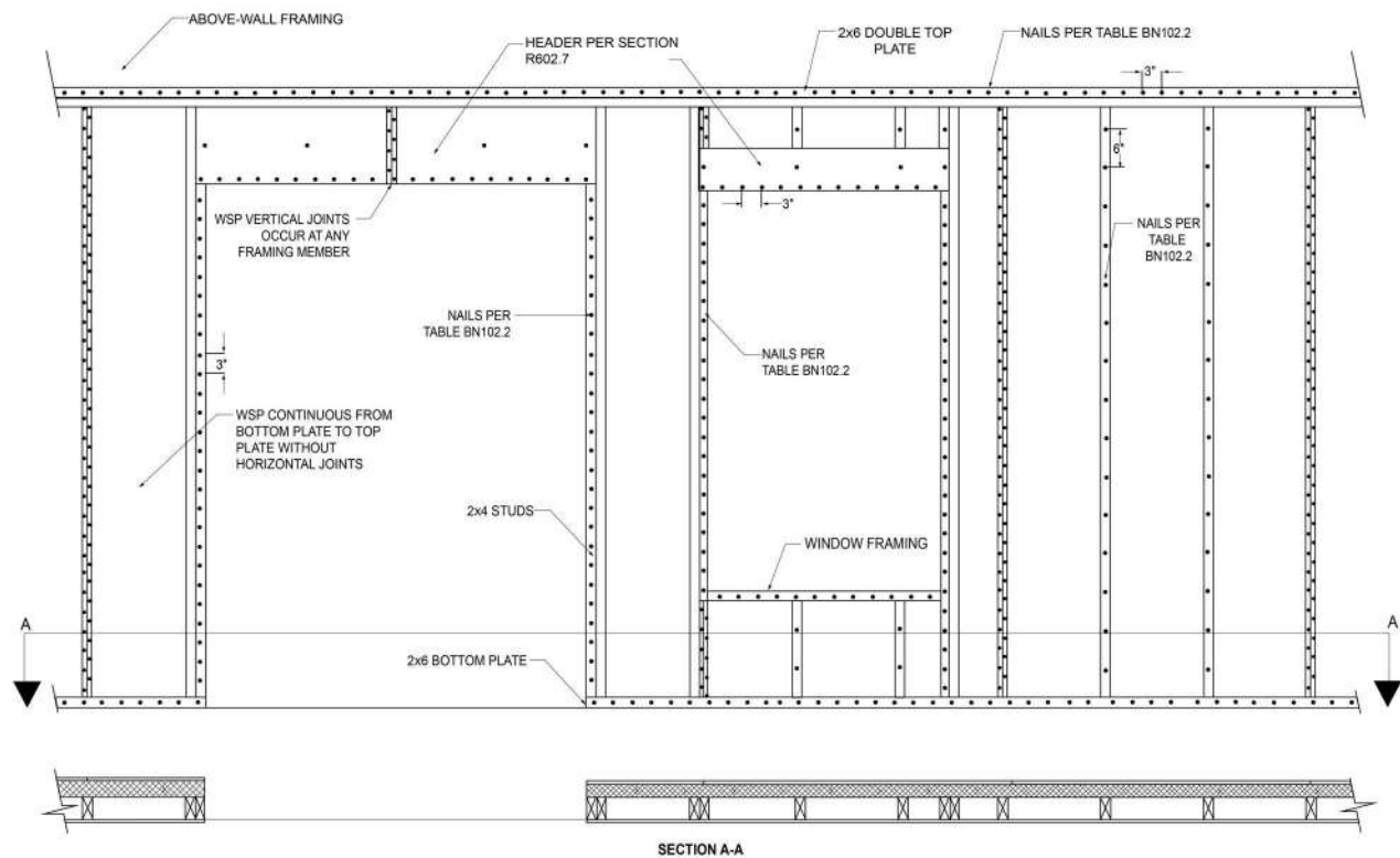
FIGURE BN102.1(2)—EXTENDED PLATE WALL, ELEVATION VIEW
