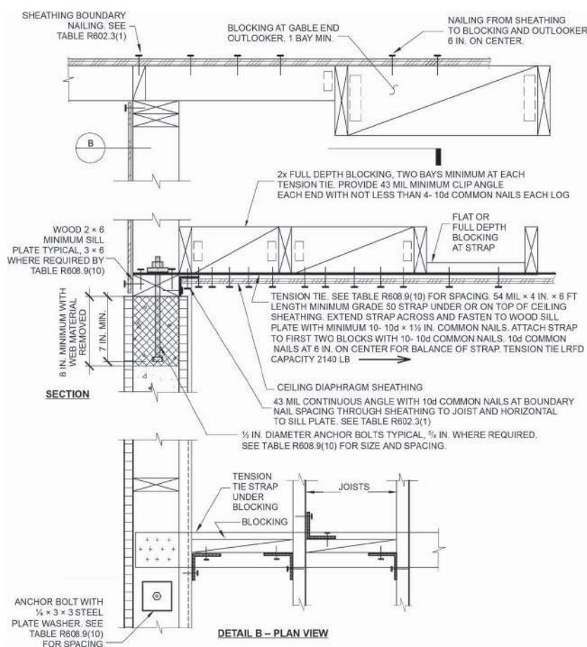
FIGURE R608.9(10)—WOOD-FRAMED ROOF TO TOP OF CONCRETE WALL, FRAMING PARALLEL
