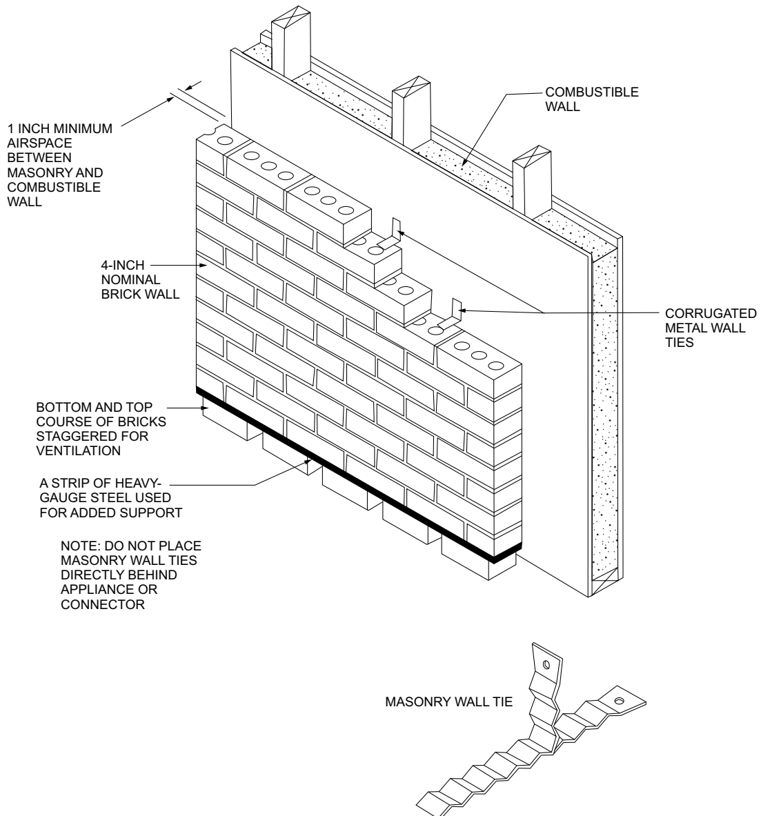
FIGURE G2409.2(3) [308.2(3)]—MASONRY CLEARANCE REDUCTION SYSTEM
