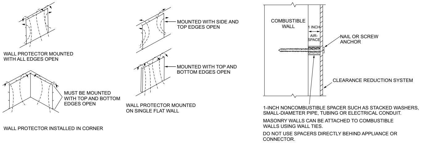
FIGURE G2409.2(2) [308.2(2)]—WALL PROTECTOR CLEARANCE REDUCTION SYSTEM
