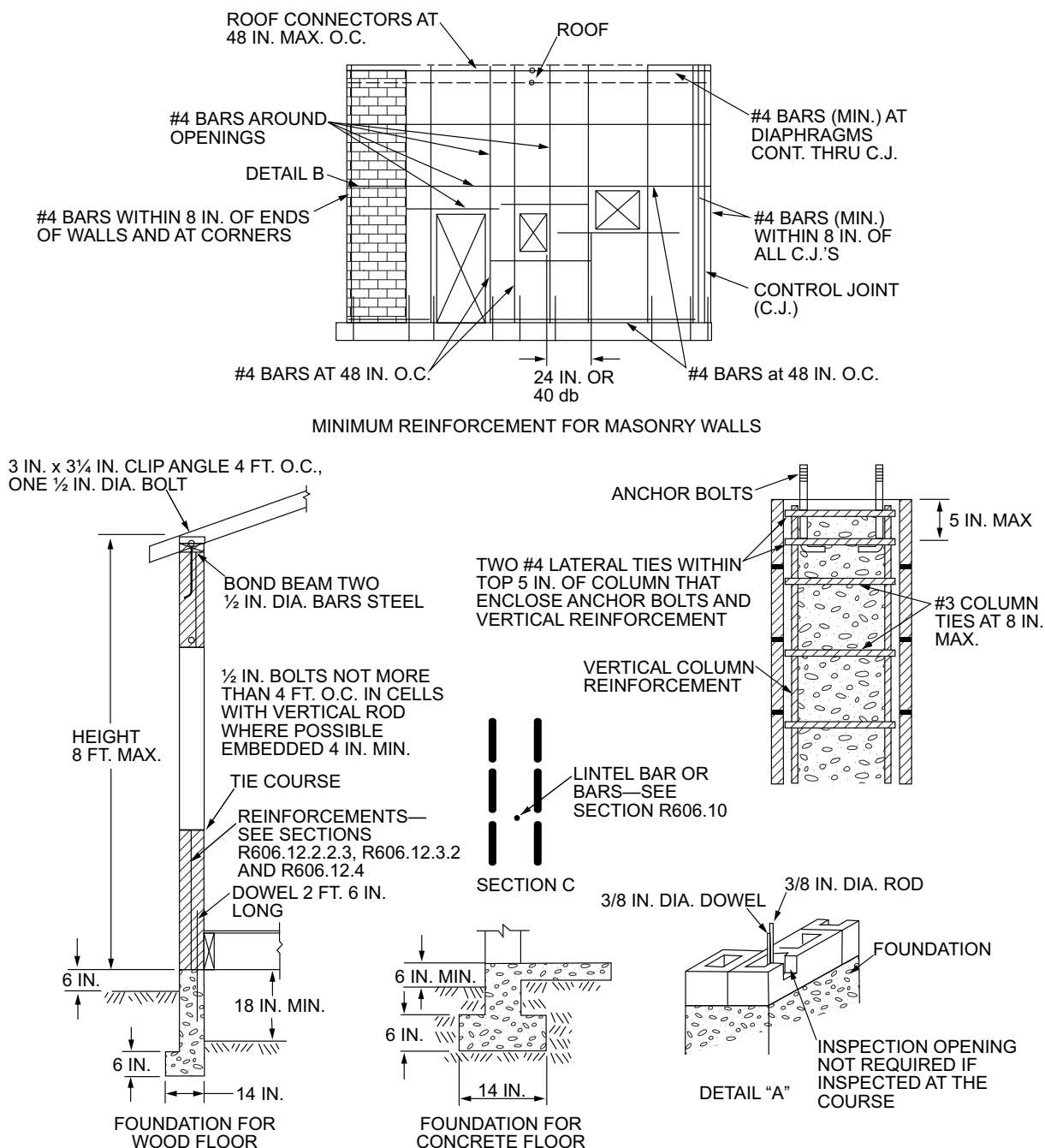
FIGURE R606.11(3)—REQUIREMENTS FOR REINFORCED MASONRY CONSTRUCTION IN SEISMIC DESIGN CATEGORY D 0 , D 1 OR D 2
