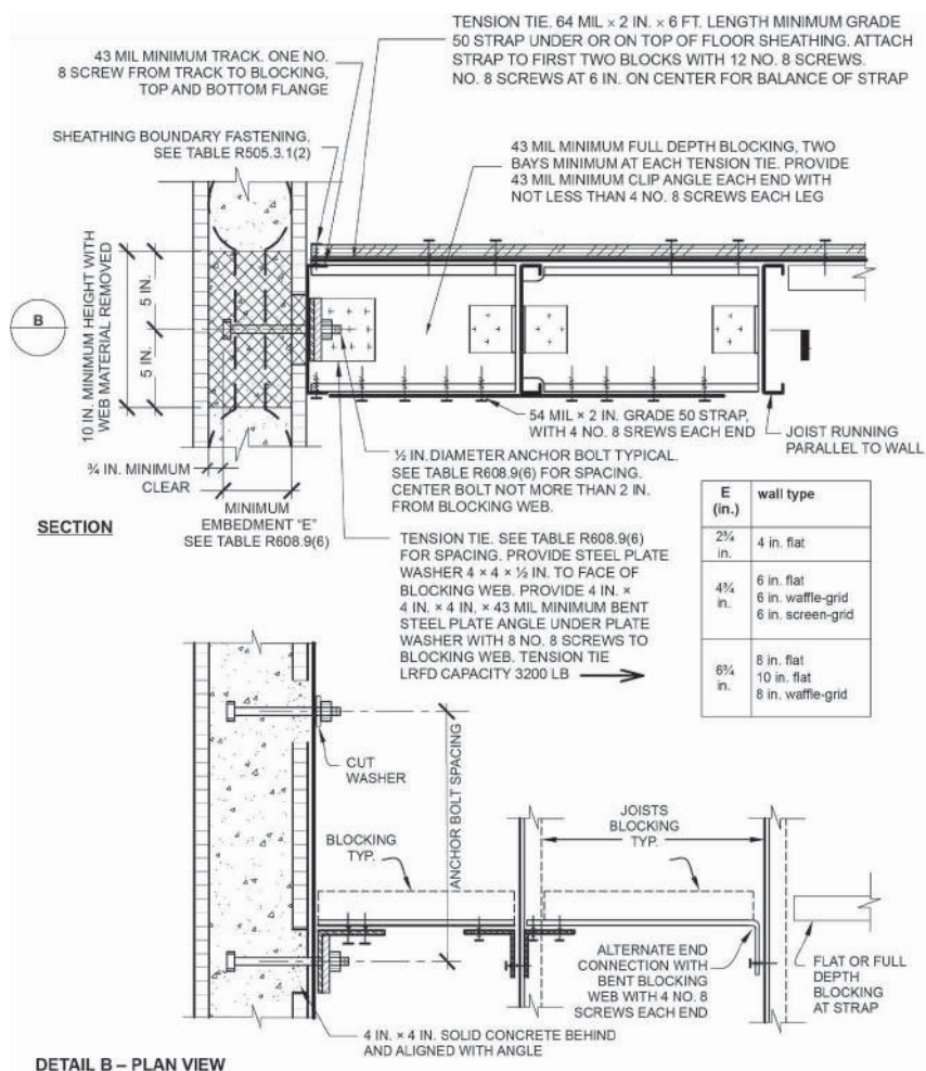
FIGURE R608.9(6)—COLD-FORMED STEEL FLOOR TO SIDE OF CONCRETE WALL, FRAMING PARALLEL
