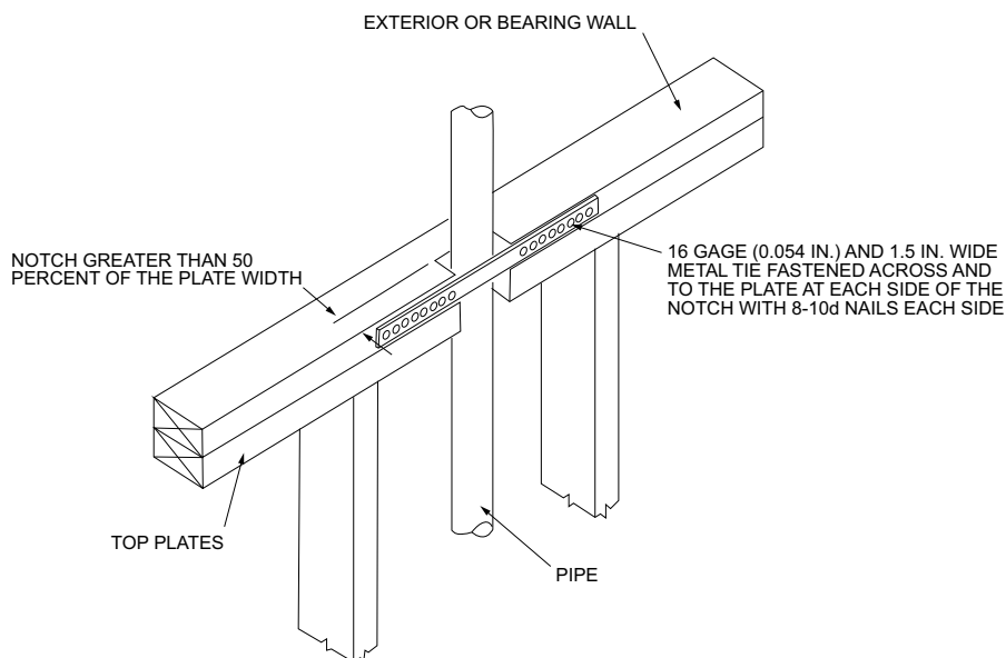
FIGURE R602.6.1—TOP PLATE FRAMING TO ACCOMMODATE PIPING
