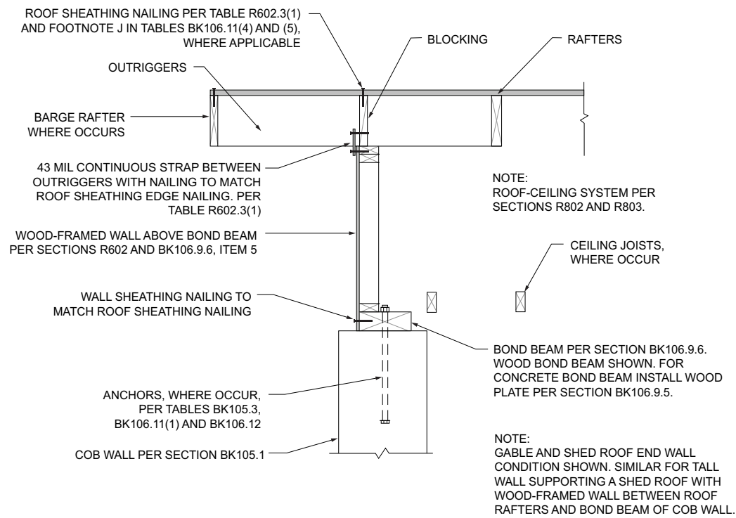
FIGURE BK106.9.6—CONNECTIONS AT GABLE AND SHED ROOF END WALLS
