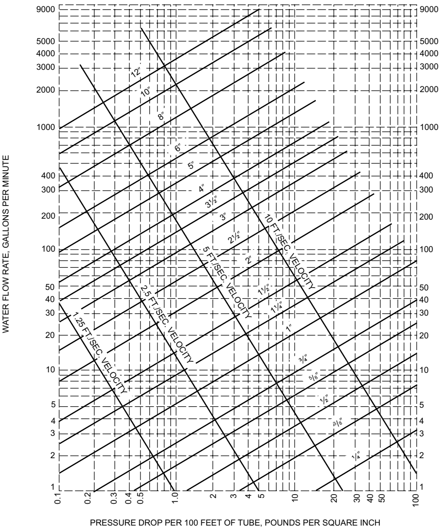
FIGURE CF103.3(3)—FRICTION LOSS IN SMOOTH PIPE a (TYPE L, ASTM B88 COPPER TUBING)
