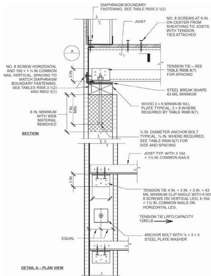
FIGURE R608.9(7)—COLD-FORMED STEEL FLOOR TO TOP OF CONCRETE WALL, FRAMING PERPENDICULAR
