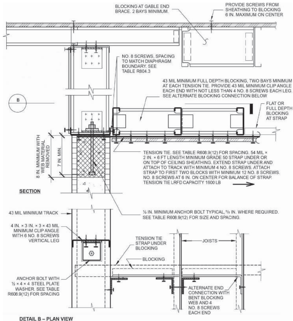
FIGURE R608.9(12)—COLD-FORMED STEEL ROOF TO TOP OF CONCRETE WALL, FRAMING PARALLEL
