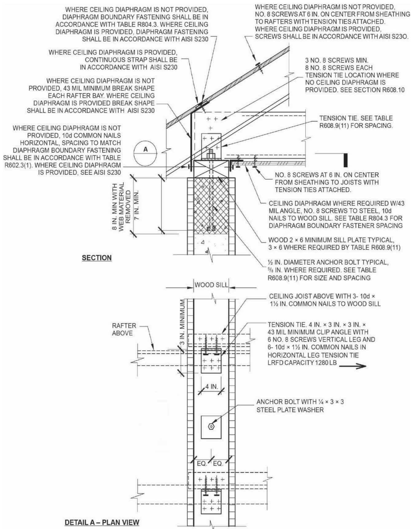
FIGURE R608.9(11)—COLD-FORMED STEEL ROOF TO TOP OF CONCRETE WALL, FRAMING PERPENDICULAR
