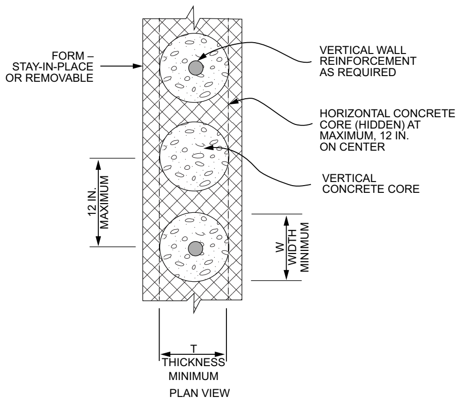
FIGURE R608.3(3)—SCREEN-GRID WALL SYSTEM
