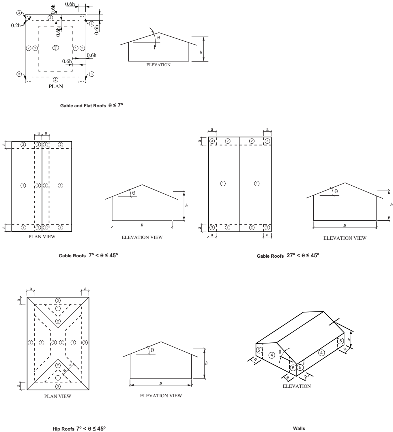
FIGURE R301.2.1—COMPONENT AND CLADDING PRESSURE ZONES
