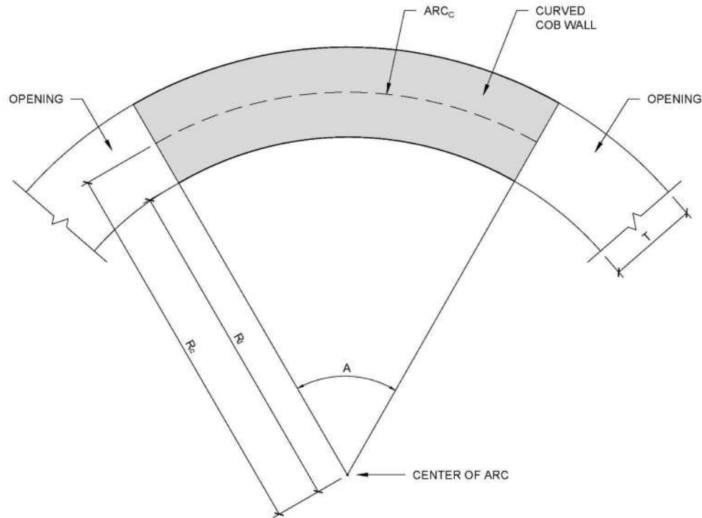
FIGURE BK106.11.3—CURVED BRACED WALL PANEL
