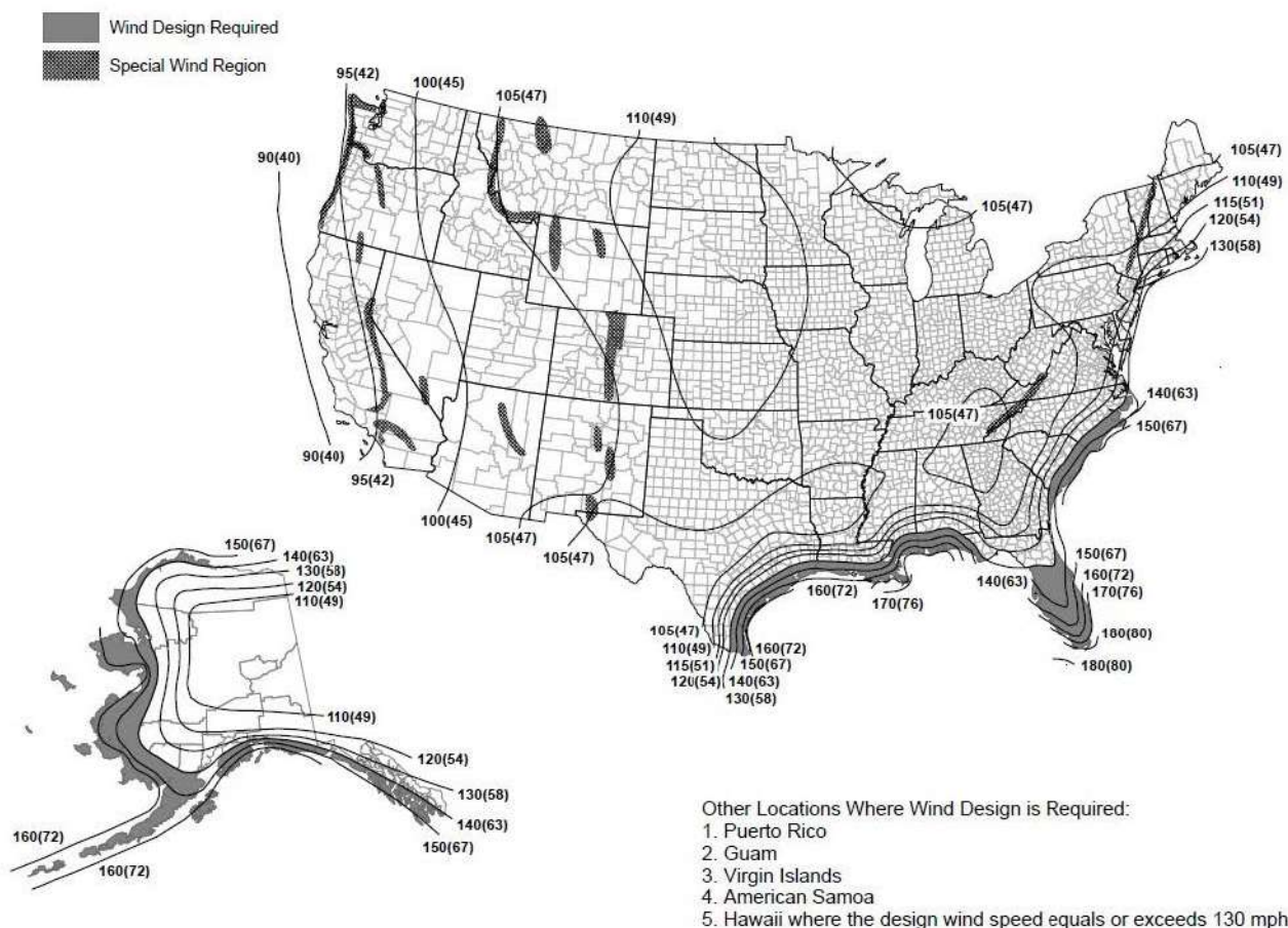
FIGURE R301.2.1.1—REGIONS WHERE WIND DESIGN IS REQUIRED
