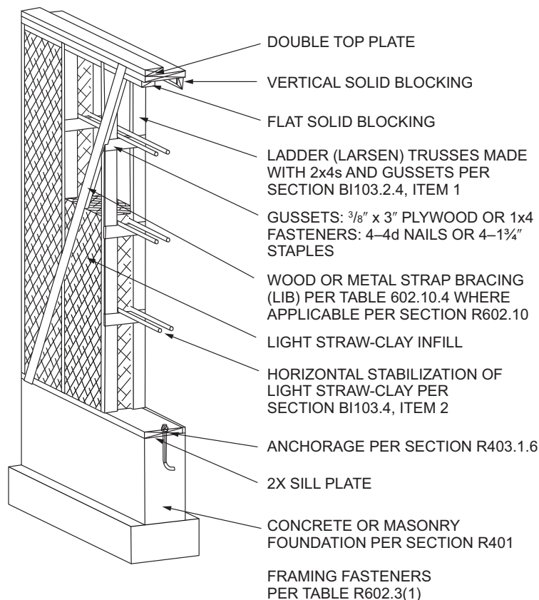
FIGURE BI103.2.4(1)—LIGHT STRAW-CLAY WALL WITH LARSEN TRUSSES
