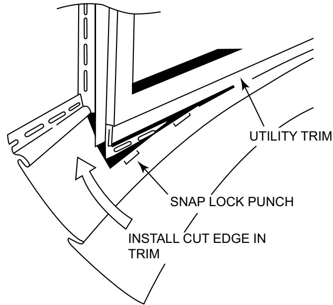
FIGURE R703.11.1.2 (2)—TYPICAL SNAP LOCK AND UTILITY TRIM UNDER WINDOW a
