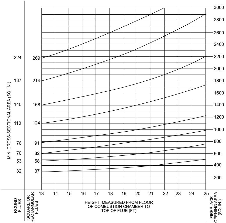
FIGURE R1003.15.2—FLUE SIZES FOR MASONRY CHIMNEYS
