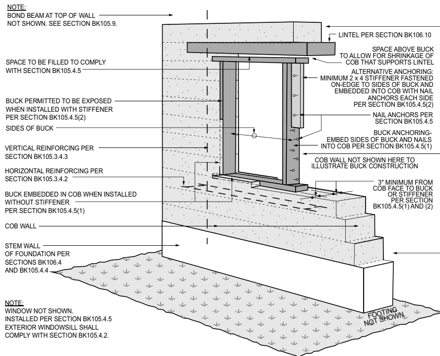
FIGURE BK105.4.5—WINDOW INSTALLATION (DOOR INSTALLATION SIMILAR)
