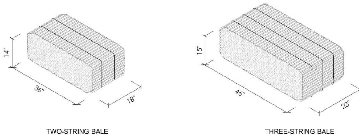
FIGURE BJ103.2—APPROXIMATE DIMENSIONS OF COMMON STRAW BALES
