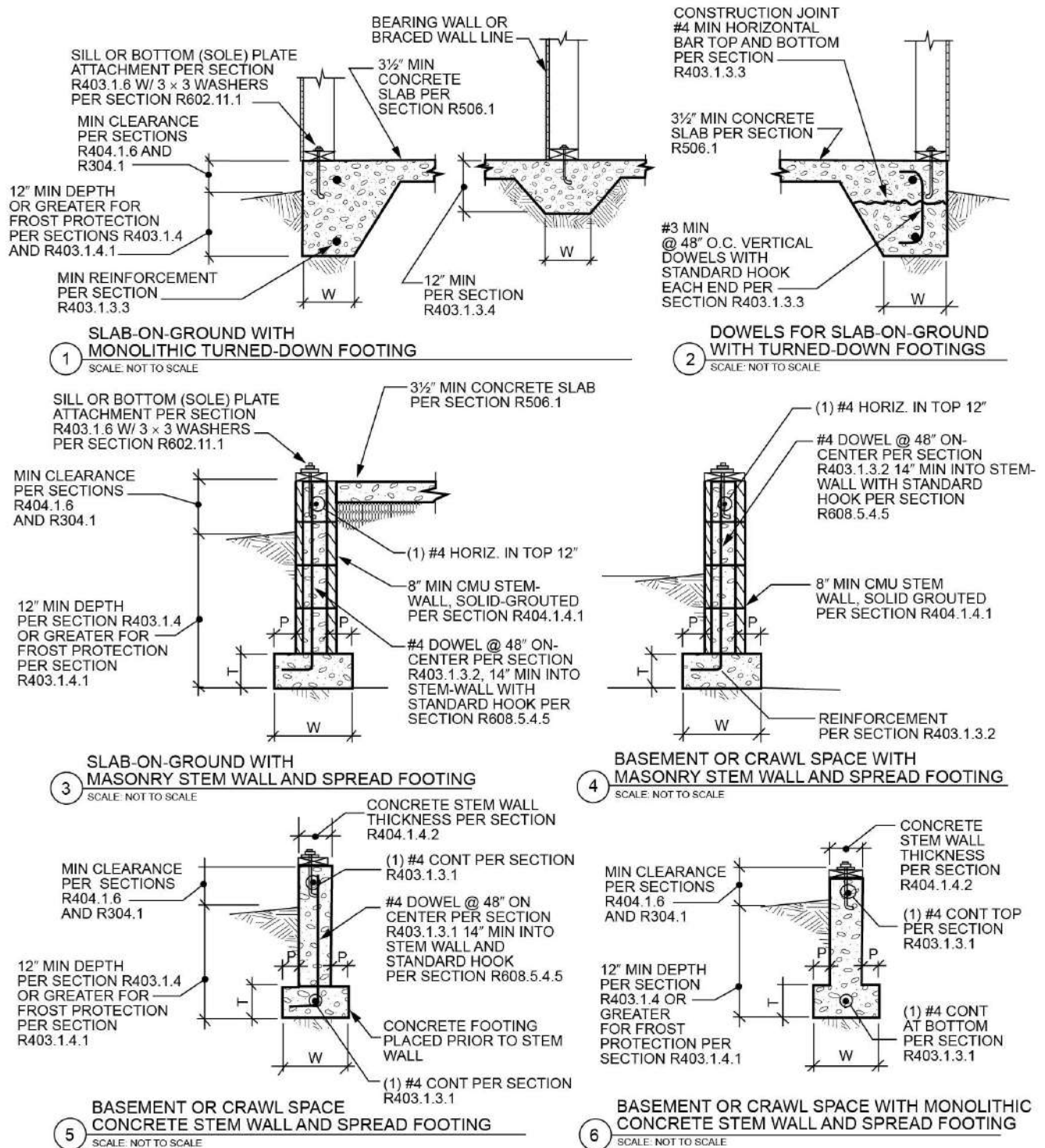
FIGURE R403.1.3—REINFORCED CONCRETE FOOTINGS AND MASONRY AND CONCRETE STEM WALLS IN SDC D 0 , D 1 AND D 2 a, b, c, d, e, f
