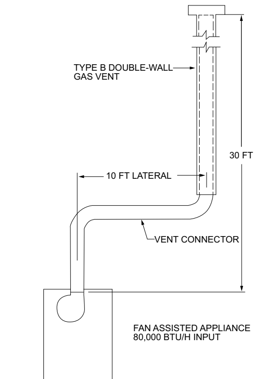
FIGURE CB101.2—EXAMPLE 2: SINGLE FAN-ASSISTED APPLIANCE
