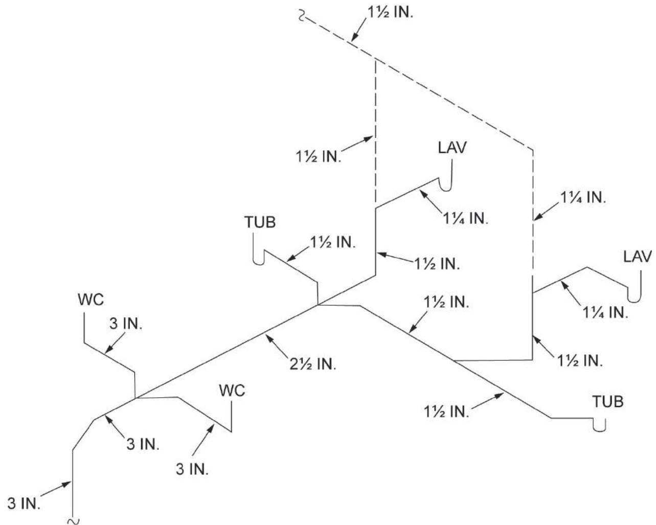
FIGURE CE101.1(3)—TYPICAL HORIZONTAL WET VENTING
