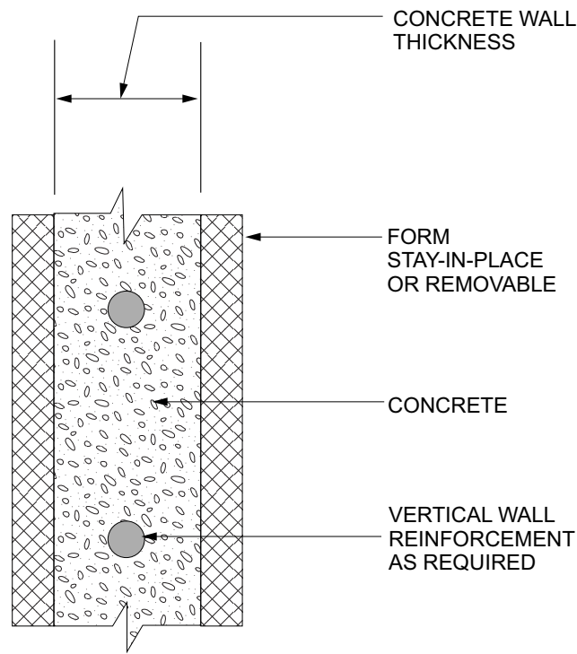
FIGURE R608.3(1)—FLAT WALL SYSTEM
