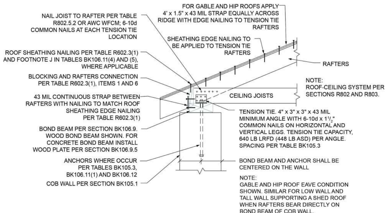
FIGURE BK106.9.5—CONNECTION OF ROOF FRAMING TO BOND BEAMS
