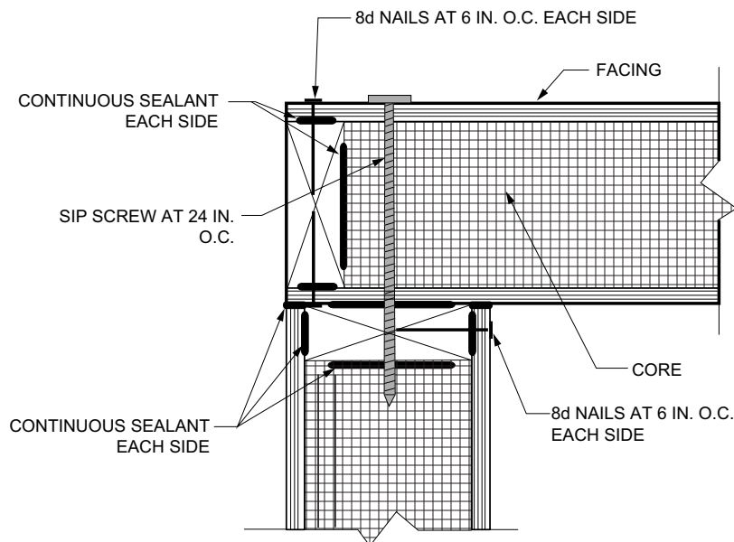
FIGURE R610.5.4—SIP CORNER FRAMING DETAIL
