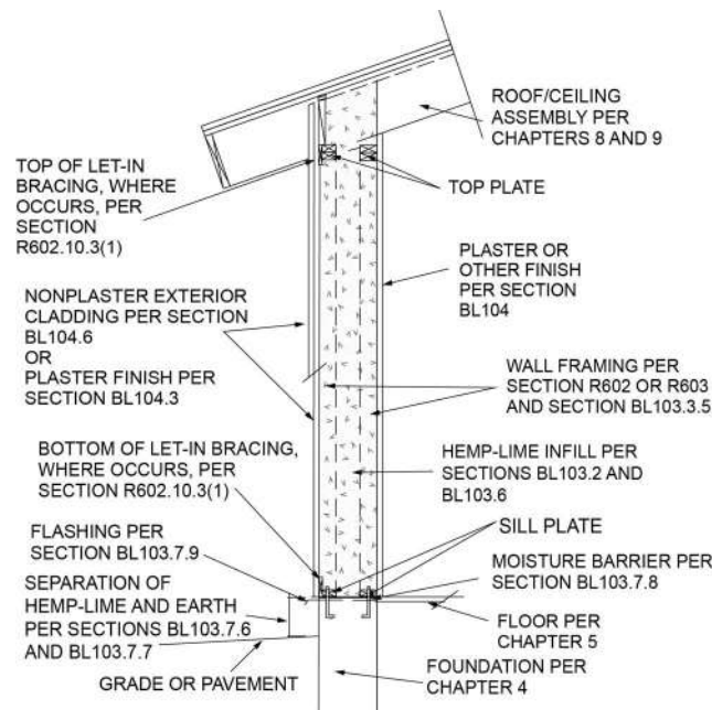
FIGURE BL103.1(4)—TYPICAL HEMP-LIME WITH DOUBLE STUD WALL FRAMING
