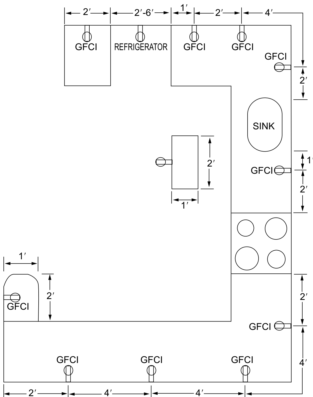
FIGURE E3901.4—COUNTERTOP RECEPTACLES
