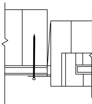
FIGURE R609.7.2(8)—THROUGH THE FLANGE
