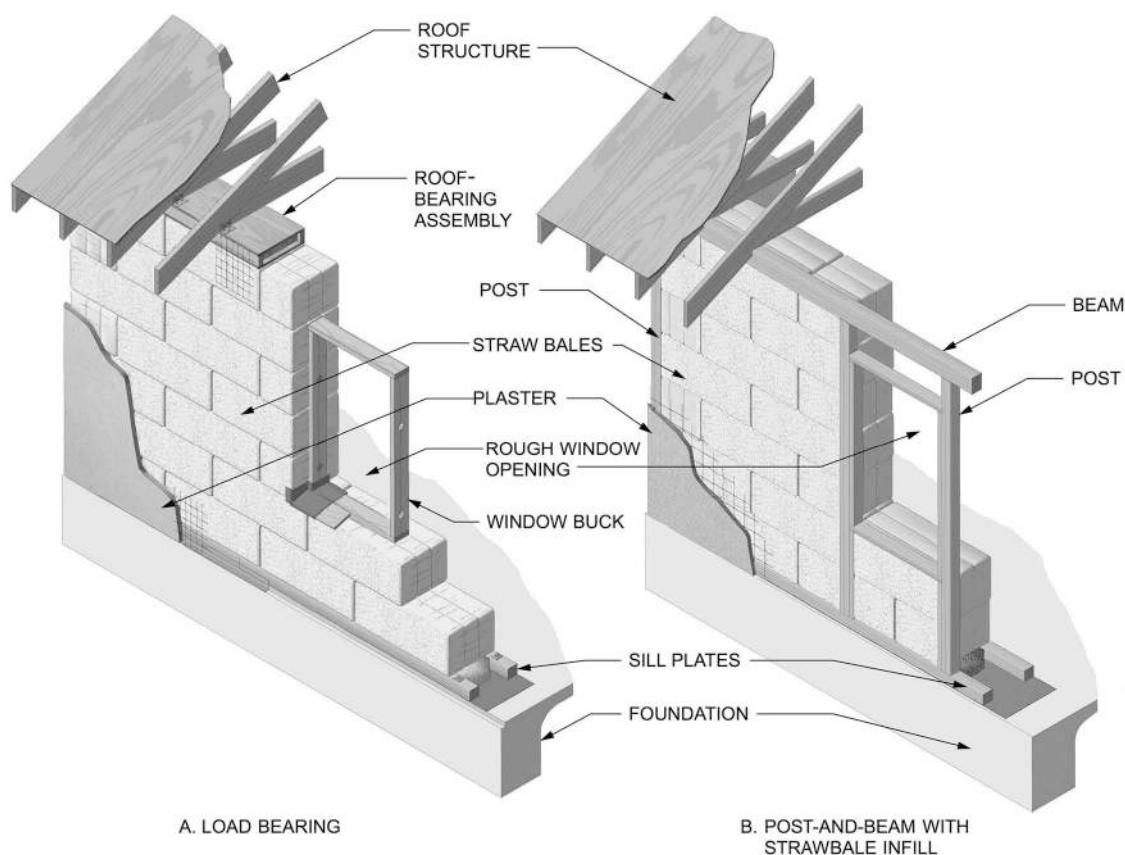
FIGURE BJ101.2—TYPICAL STRAWBALE WALL SYSTEMS
