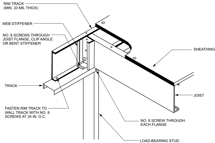
FIGURE R505.3.1(1)—FLOOR-TO-EXTERIOR LOAD-BEARING WALL STUD CONNECTION
