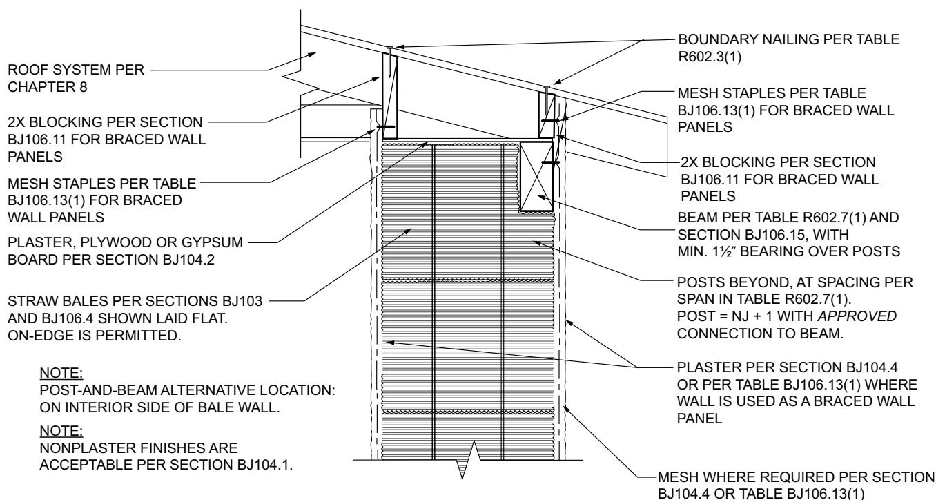
FIGURE BJ105.1(4)—TYPICAL TOP OF POST-AND-BEAM WALL WITH PLASTERED STRAWBALE INFILL
