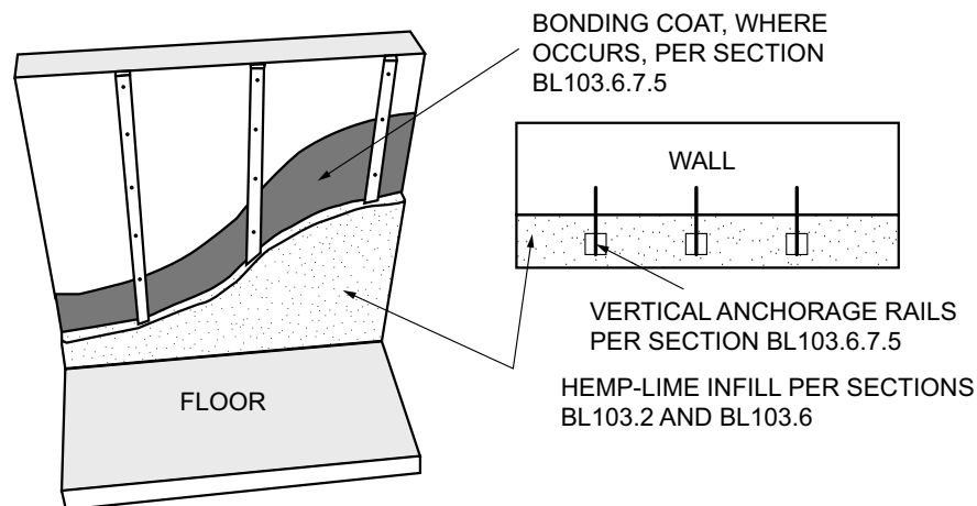
FIGURE BL103.6.7.5—TYPICAL HEMP-LIME THICK LINING
