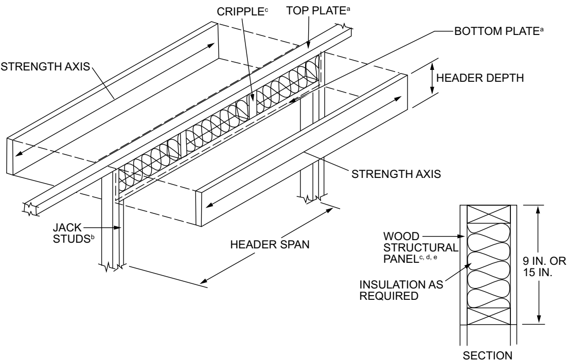
FIGURE R602.7.3—TYPICAL WOOD STRUCTURAL PANEL BOX HEADER CONSTRUCTION
