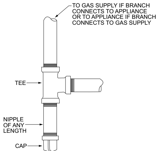
FIGURE G2419.4 (408.4)—METHOD OF INSTALLING A TEE FITTING SEDIMENT TRAP
